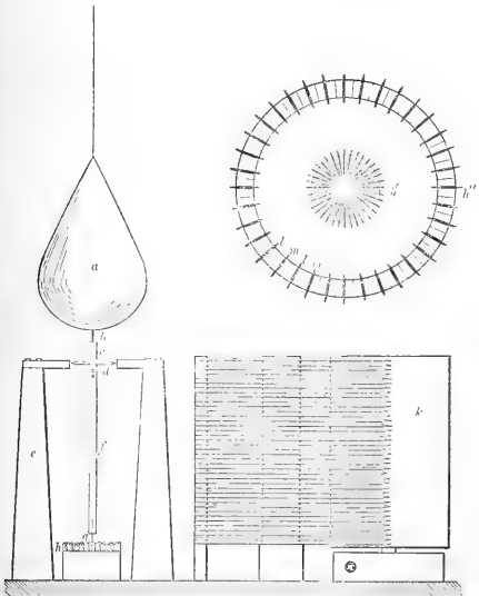
FIG. 3.—Azimuth register of wave path in all phases of an earthquake.
