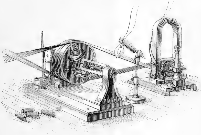
Smith's Transmission Ergometer.
