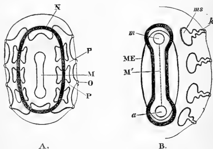
Sedgwick's theory of segmentation: A. Ideal ancestor of segmented animals; B. Invertebrate.— N , primitive mouth; m , mouth; a , anus; M' , middle portion of primitive mouth or blastopore closed up; N , nervous system; p , pouch of gut; ms , mesoblastic somite; k , nephridium; o , external pore; ME , mesenteron.
