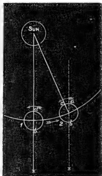
Fig. 49.—Diagram showing how the difference between the lengths of the sidereal and mean day arises.
