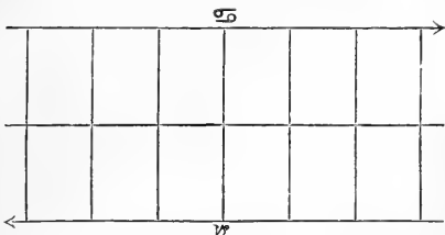
FIG. 51.—Diagram showing how the sun's apparent motion along the ecliptic, now parallel with the earth's equator (the central line of the figure) at the summer ( \tau ) and winter ( \omega ) solstices, is represented by equal intervals along the equator.
