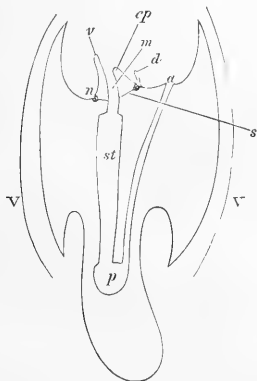
Diagram of body plan of Brachiopod , Polyzoan , and Phoronis (after Caldwell)— m , mouth; a , anus; s , septum; n , nervous system; st , stomach; F , second stomach; ep , epistome; v , tentacle of ventral series; d , tentacle of dorsal series; V valves of Brachiopod skull.
