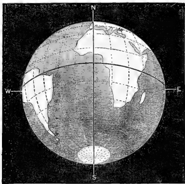
FIG. 45.—The earth, as seen from the sun at the winter solstice (noon at London).
