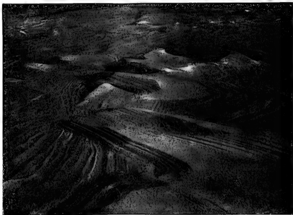
FIG. 3.—Stratification of Snow revealed by Wind Erosion.
