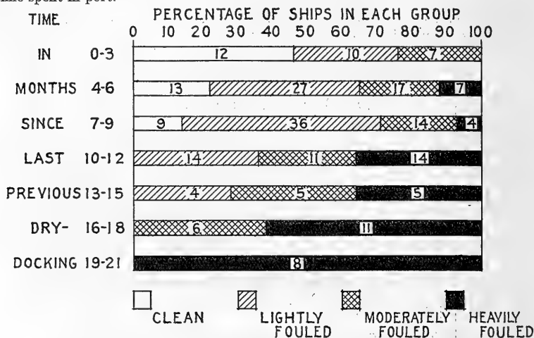
FIG. 25.—Relation between amount of fouling and amount of time between dry dockings
