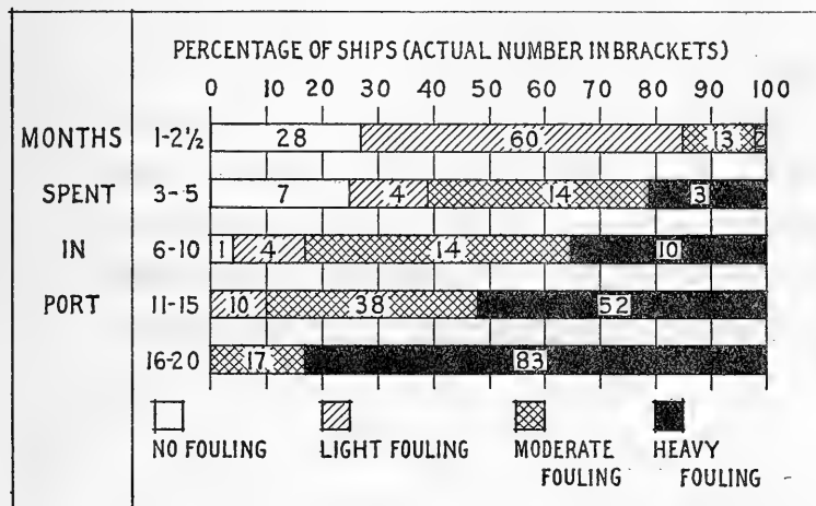
FIG. 25.—Relation between the degree of fouling and the amount of time spent in port between dry dockings
