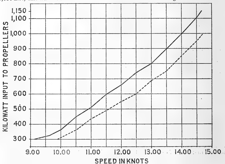
FIG. 22.—U. S. Submarine S-54 . Standardization trials, measured mile. Provincetown, Mass., May 16-18, 1923. Vessel out of dock 56 days for run with foul bottom. Motor efficiency disregarded as virtually constant. — with foul bottom; - - - - with clean bottom
