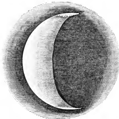
FIG. 2.—Details of snow-caps January 19, 1878 (Trouvelot).
