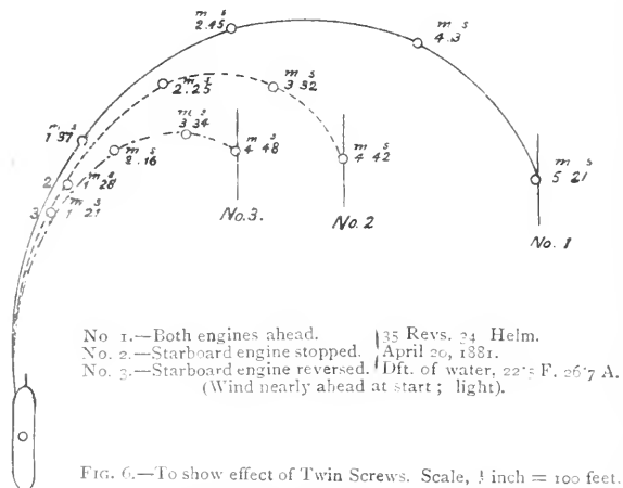
FIG. 6.—To show effect of Twin Screws. Scale, ¼ inch = 100 feet.
