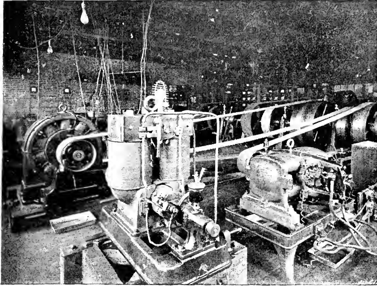
FIG. 1.—Dynamometer Room.
