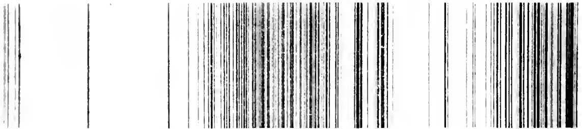
Fig. 3. Photograph of a portion of the infrared solar spectrum lying between wave-lengths 1.4\mu and 2.2\mu .
