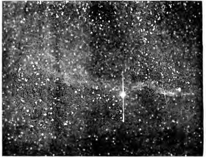
FIG. 13.—The nebula near \epsilon Cygni, from a photograph by Dr. Roberts
