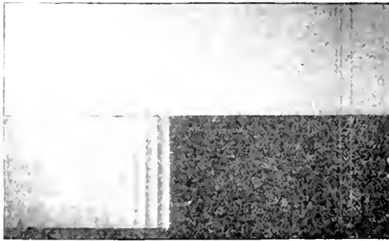
Fig. 17. Spectrum of magnesium at the lowest temperature at which we can get any light from it.
