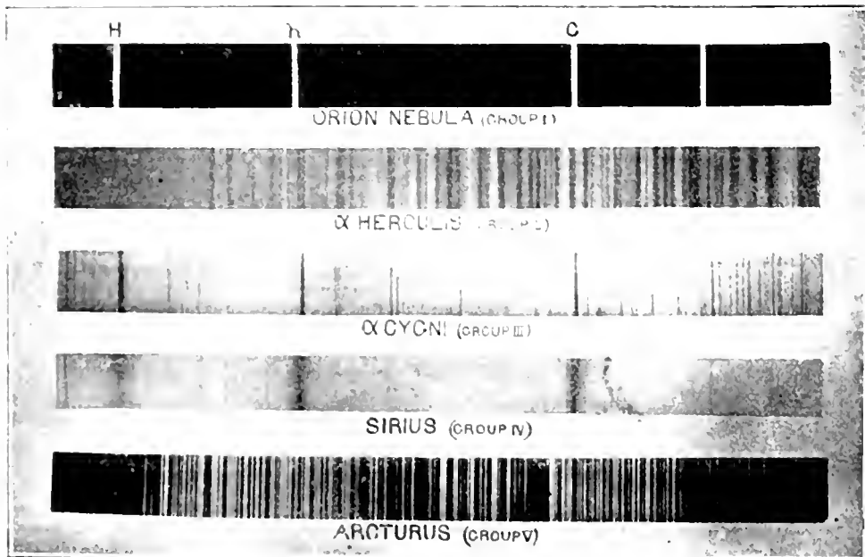
Fig. 1. The photographed spectrum of a nebula contrasted with the spectra of stars.
