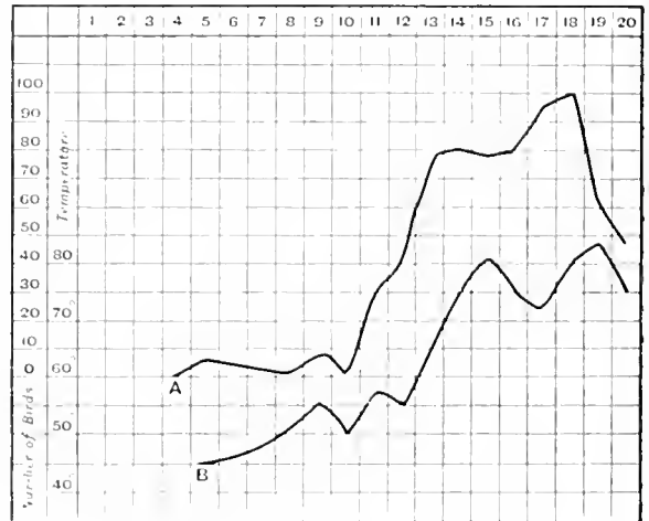
FIG. 1.—A, Migration Curve; T, Temperature Curve.
