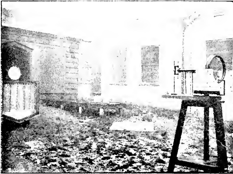
FIG. 16.—Showing obliquity of horizontal telescope used with siderostat.
