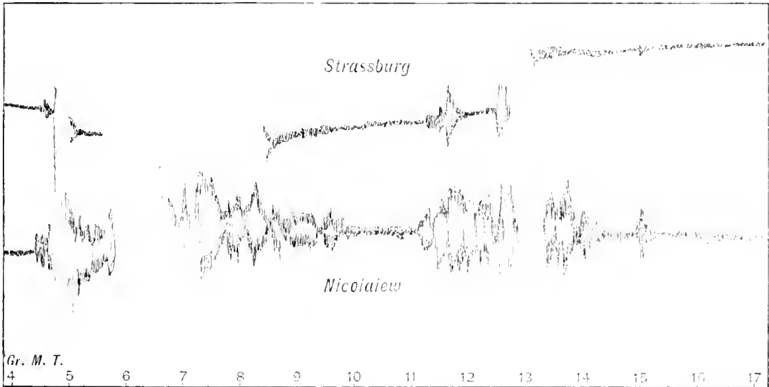
FIG. 1.—Earthquake Disturbance observed at Strassburg and at Nicolaiew on June 11, 1894.
