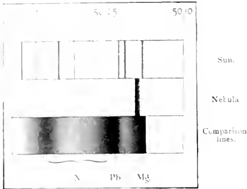
FIG. 20.—N and position of the chief nebular line, according to Keeler.
