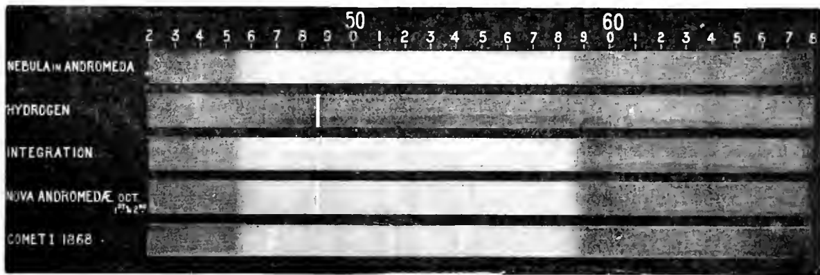
FIG. 12.—Spectrum of the nebula in Andromeda compared with Nova Andromedæ and comet. The flatings common to all are those of carbon.
