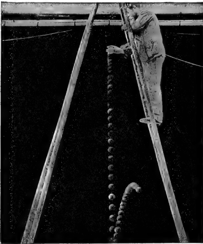
FIG. 11.—Series of positions taken up by a falling ball studied by chronophotography on a fixed plate.
