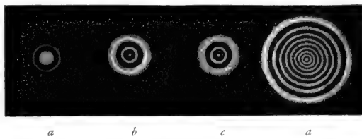
FIG. 1.—Diagrams showing spurious disk and diffraction rings seen with a perfect objective.
