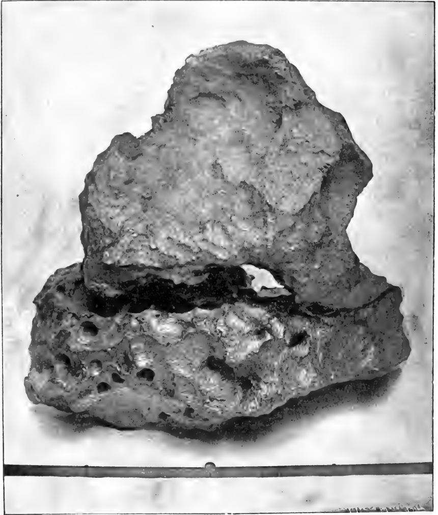
FIG. 1.—General appearance of meteorite.
