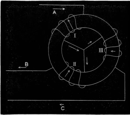
FIG. 20.—Three-phase alternate current motor (open winding); currents differing by 120^\circ in phase, and represented in direction and magnitude by the direction and length of the arrows.
