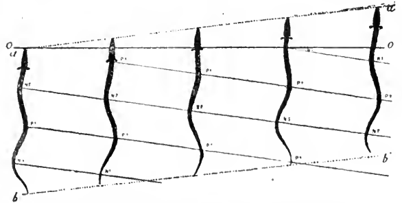
FIG. 8.—Eel swimming in a horizontal plane. The horizontal line oo shows plainly the inclination of those lines which join the crests and troughs of the waves formed by the body, so that the velocity of progression of the animal is expressed by the inclination of the line oa .
