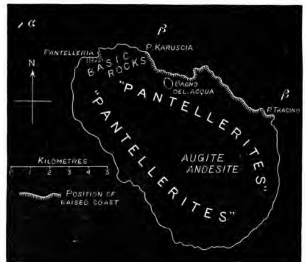
FIG. 1.—Map of Pantelleria, showing the position, according to Ricco, of (a) the submarine eruption of October 1891, and (b, β) of the raised coast.
