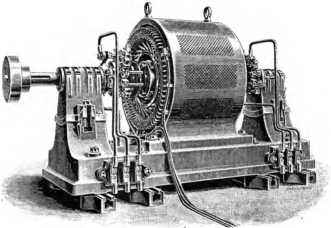
Fig. 32.—The Frankfort 100 horse-power rotatory current motor.
