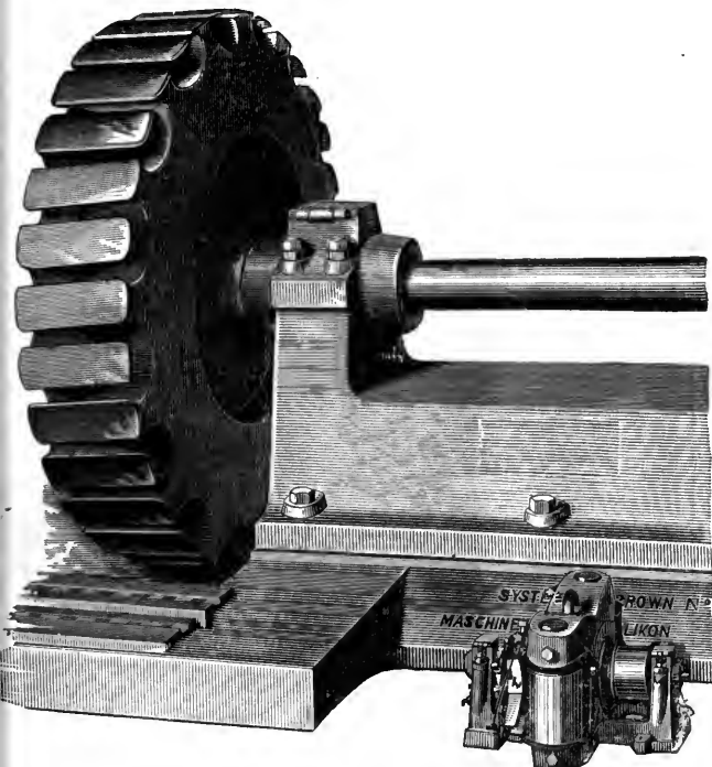
FIG. 34.—Field magnet of the Lauffen three-phase alternate current dynamo.
