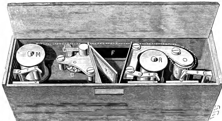
FIG. 5.—The chamber in which the images are formed, with the lid raised. M and R are the drums on which the films are rolled off and on respectively; r , r , r , small rollers pressing the film on the cylinders; L , the driver, with its pressing cylinder; F , the aperture for the admission of the image; v , ground glass with hinged motion. The dotted line indicates the path of the band of film; c ' and c , the clamber and its cam, which produces the intermittent action of this band.
