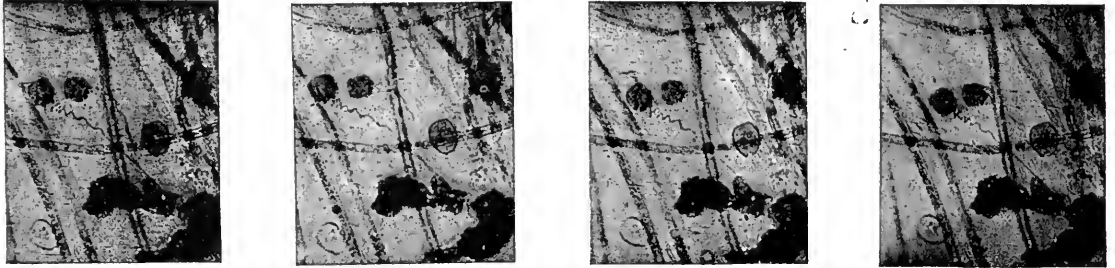
FIG. 10.—Showing the movements of Vorticellæ. The phases of movements must be read from left to right.
