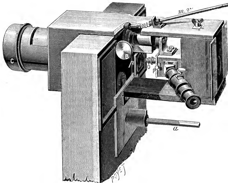
FIG. 9.—Special piece of apparatus for studying the movements of microscopical objects.
