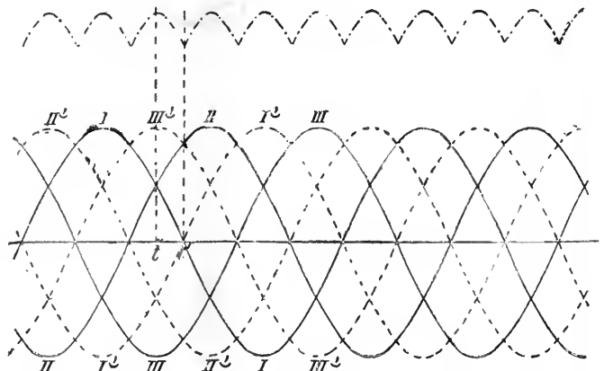
FIG. 23.—Three harmonic alternating currents of the same period and maximum altitude, but differing by 120^\circ in phase.
