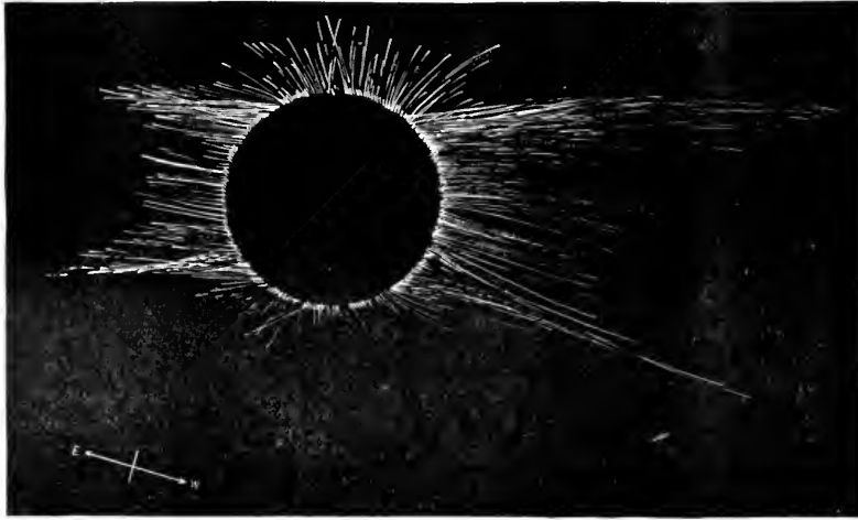
FIG. 1.—Prof. Engler's sketch of corona, 1889.
