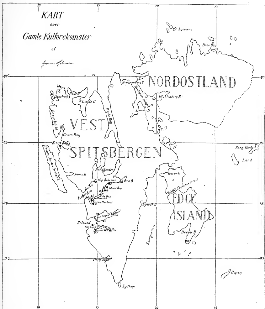
Fig. 2. Kart over Spitsbergens kulforekomster.
