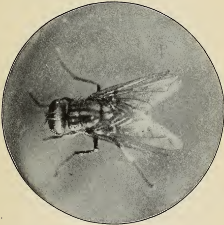
FIG. 65. House-fly. (Photomicrograph.)
