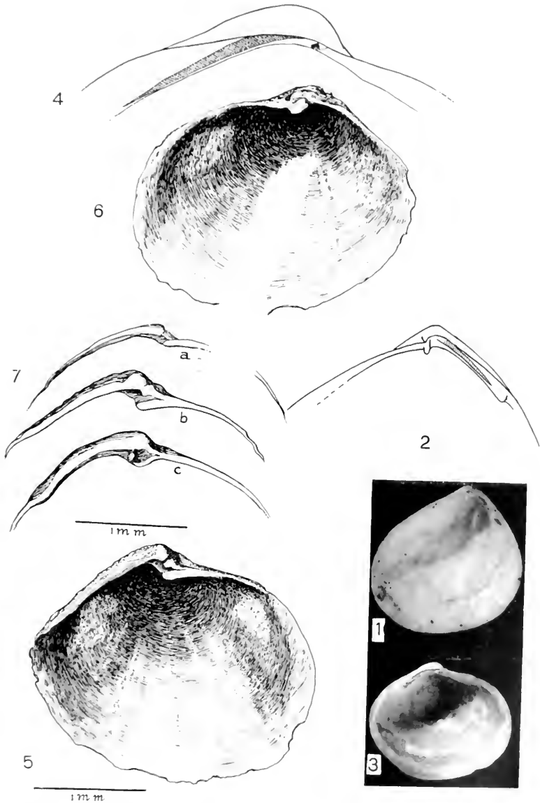
Fig. 1, Nautilus corrutusis Arnold, type; 2, hinge of right valve. 3, N. nuxea Dall, type; 4, hinge of left valve. 5, N. redondoensis , type, left valve; 6, right valve; 7, a-c, range of hinge variation.
