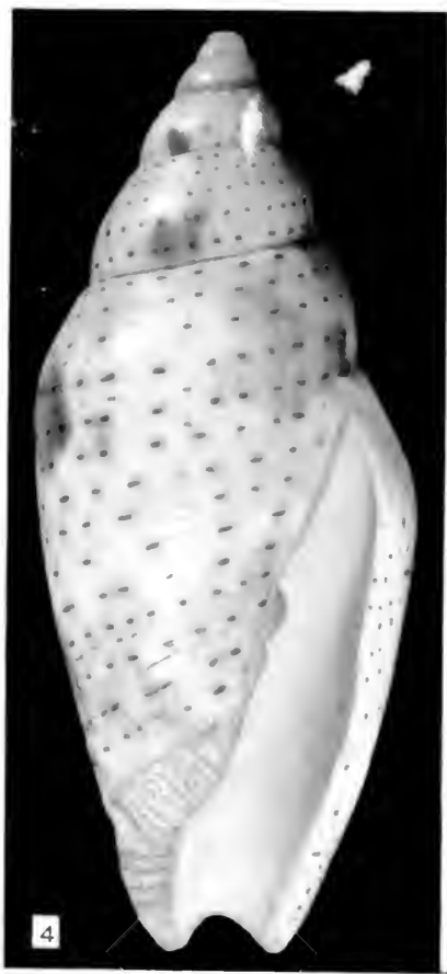
Fig. 1, tooth of Foluta scapha Gmel. (after Tryon). Fig. 2, teeth of Mitra cornua Lam. (after Tryon). Fig. 3, teeth of Mitra florida . Figs. 4, 5, Mitra florida , enlarged.
