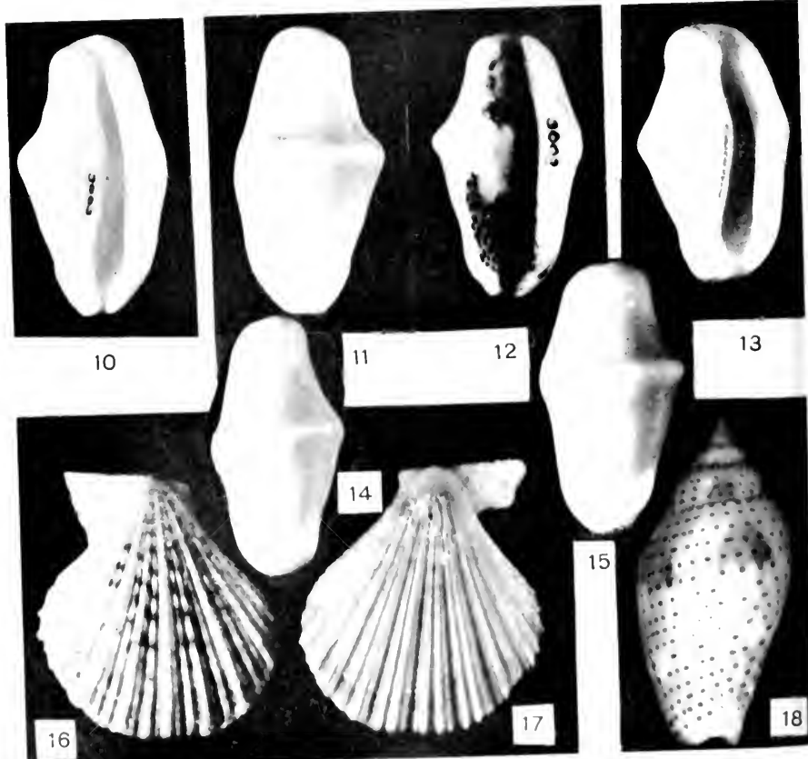
Figs. 1-5, Lobosia pulchra ; 6, 7, Margarita hutchinsoni , S. Sa, Japonia musiva. 8, Favoschelus scapharus . 10-15, Cyphoma acgypti robustior . 16, 17, Pecten imbricatus mikkolidae . 18, Mitra florida .
