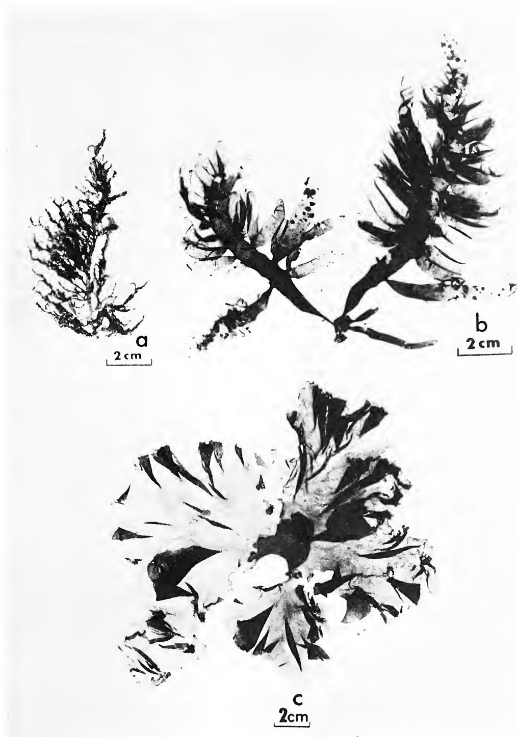
FIGURE 6.—Habits: a , Bonnemaisonia hamifera from Roca Blanca, Puerto Refugio (JN-5802); b , Botryocladia hancockii collected off Isla Mejia, Puerto Refugio (JN-5685); c , Predaea masonii from Roca Blanca, Puerto Refugio (JN-5295), showing the deeply divided blade.
