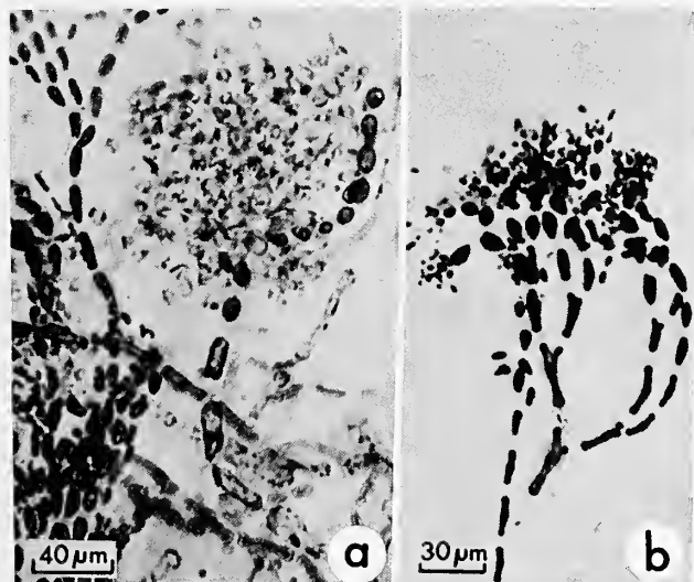
FIGURE 8.— Dudresnaya colombiana from Isla Estanque (JN-5480 ♀; ♂): a, intercalary position of cystocarp borne on the auxiliary cell; b, spermatia clustered terminally on the end of the lateral filament.
