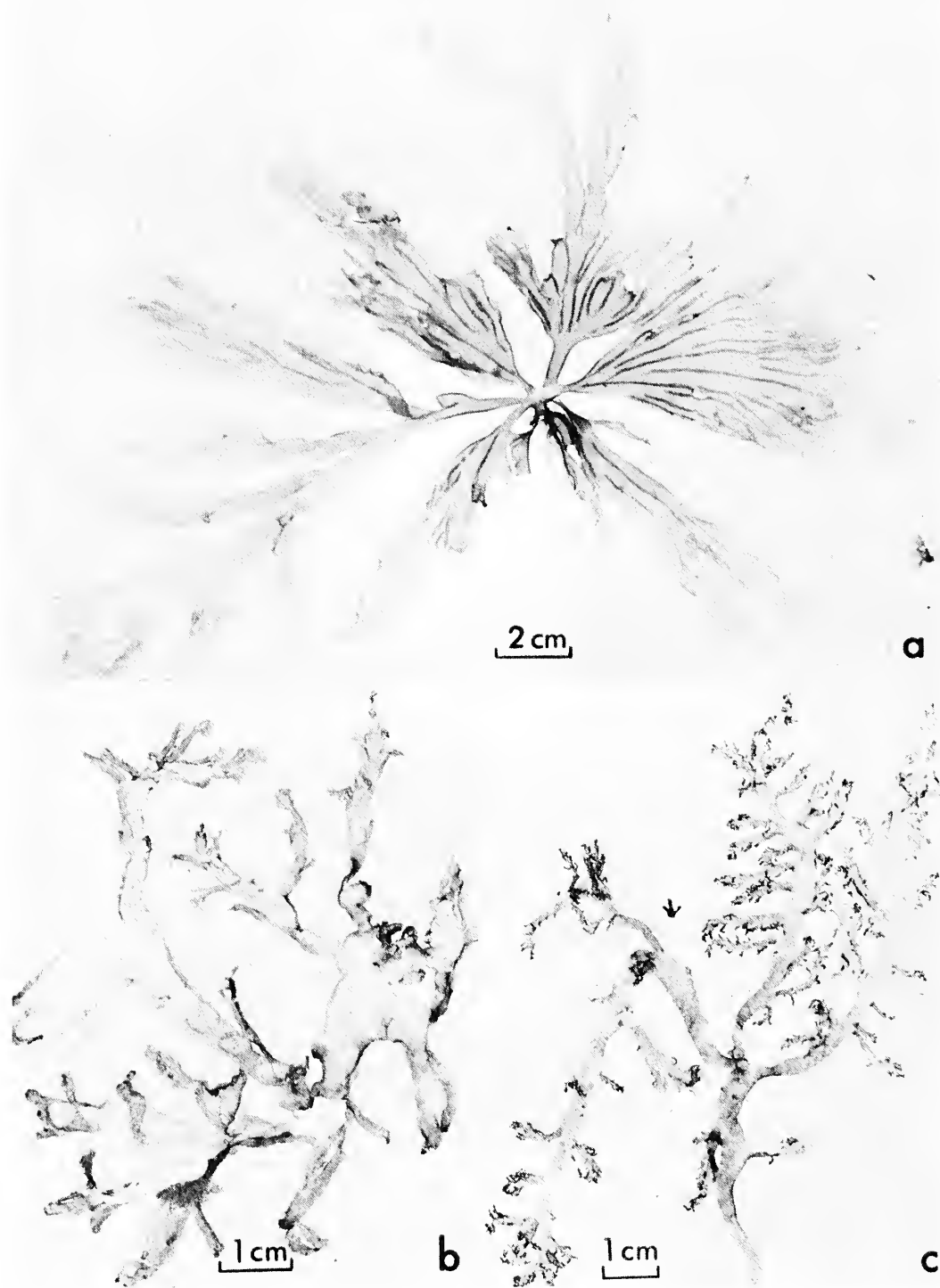
FIGURE 7.— Dudresnaya colombiana showing variation in branching: a , large specimen from Isla Mejía (JN-5680) branching of 1-2 orders and mostly from the lower portion of the thallus; b , c , smaller plants collected off Isla Estanque (JN-5480) with more numerous branches.
