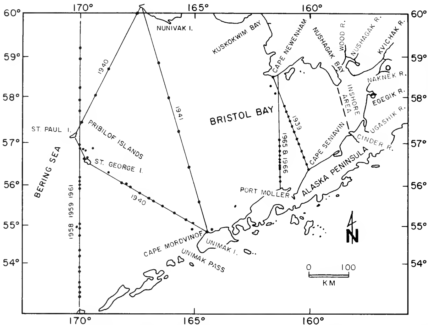
Figure 2.—Transects in the eastern Bering Sea and outer Bristol Bay where exploratory fishing was carried out in the 8 yr selected for study to determine the distribution of sockeye salmon in offshore area of Bristol Bay. (See Appendix Table 1 for source of data.)
