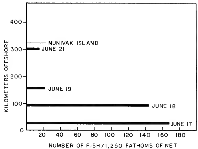
Figure 7.—Gill net catches of sockeye salmon between Pribilof Islands and Nunivak Island, 17-21 June 1940. Note: Fishing time was not specified, but I assumed that it was the same for each set. (See Appendix Table 1 for source of data.)
