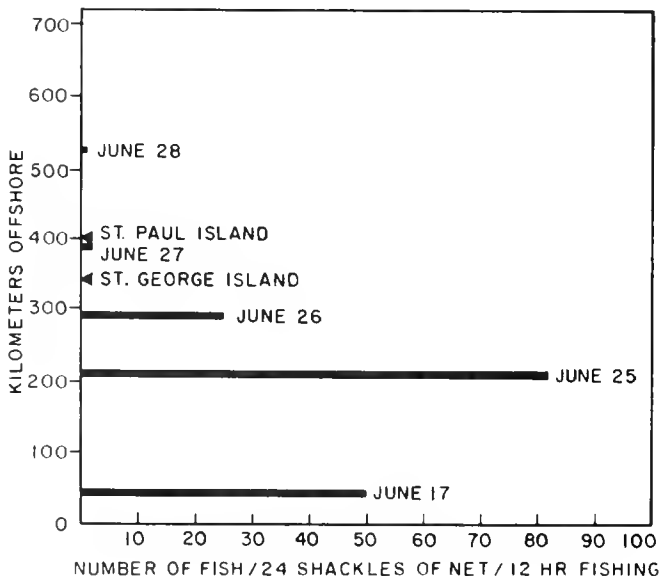
Figure 3.—Gill net catches of sockeye salmon along approximately long. 170°W, 17-28 June 1958. Each shackle of net was about 50 fathoms. (See Appendix Table 1 for source of data.)
