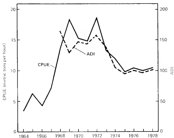
Figure 3.—Trends in catch per unit effort (CPUE) and average density index (ADI) for walleye pollock in the eastern Bering Sea, 1964-78.
