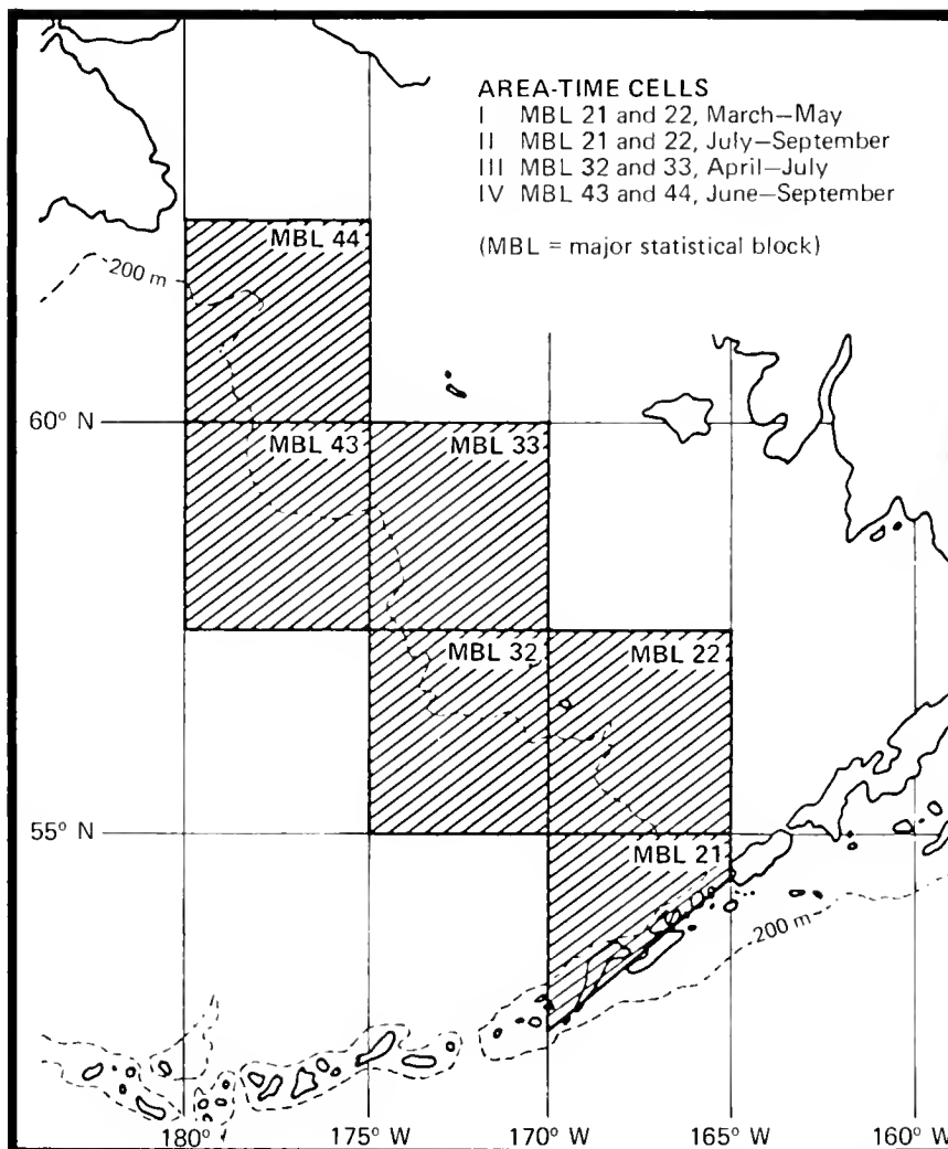
Figure 2.—Four area-time cells used for calculating average density indices for walleye pollock in the eastern Bering Sea.
