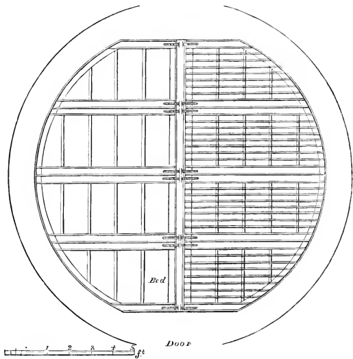
PLAN OF THE STABLES AT TEDWORTH.
