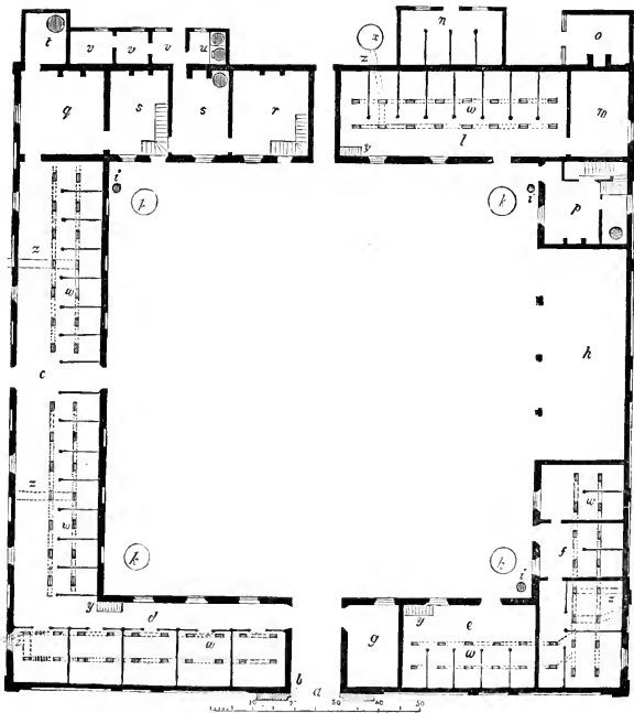
PLAN OF THE STABLES AT TEDWORTH.
