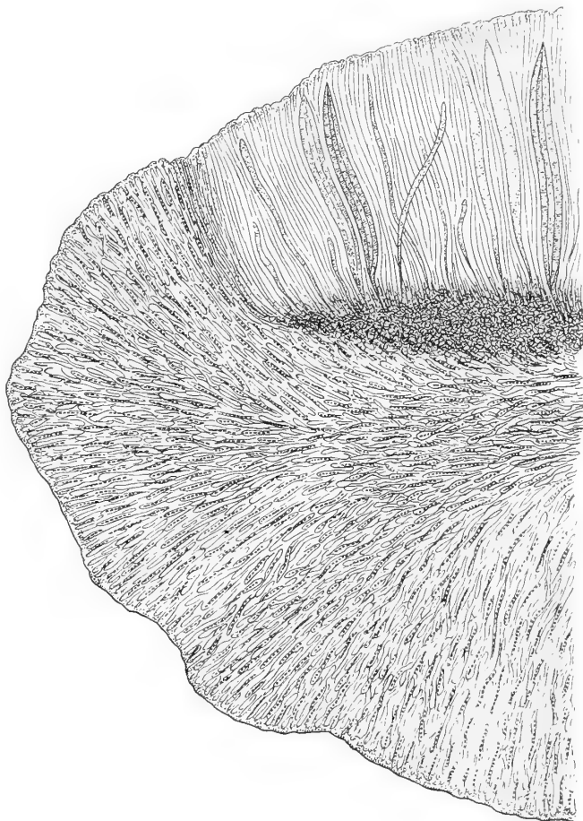
Fig. 41. — Lecideia rosella Ach.
