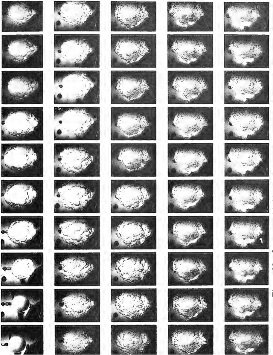
Figure 25. Sequence of bubble development from a 2-inch OD sphere. Duration of this phase, approximately 100 \mu sec.
