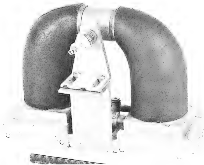
Figure 15. Arrangement for studying effect of magnetic field upon spark gap (keeper in place).
