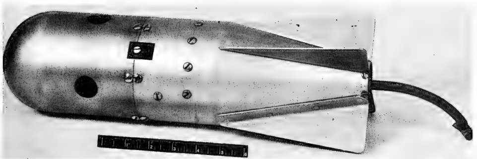
Figure 35. Original model of acoustic bomb.
