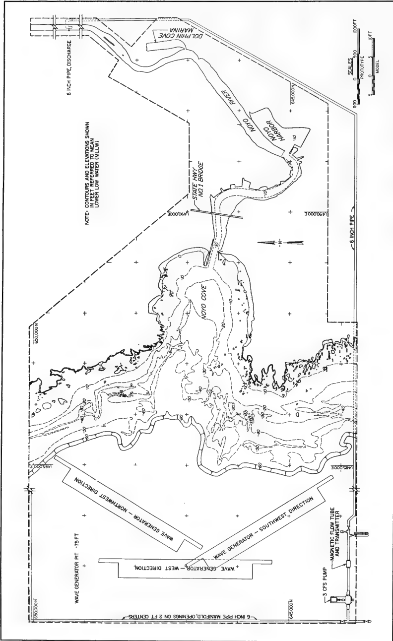
Figure 3. Model layout
