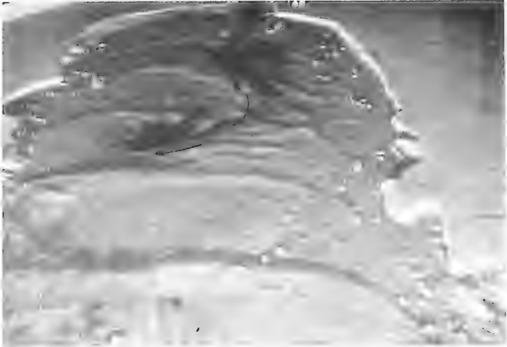
Photo 63. Riverine sediment tracer patterns for existing conditions; 15-sec, 20-ft waves from west; swl = 0.0 ft, 20,000-cfs river discharge
