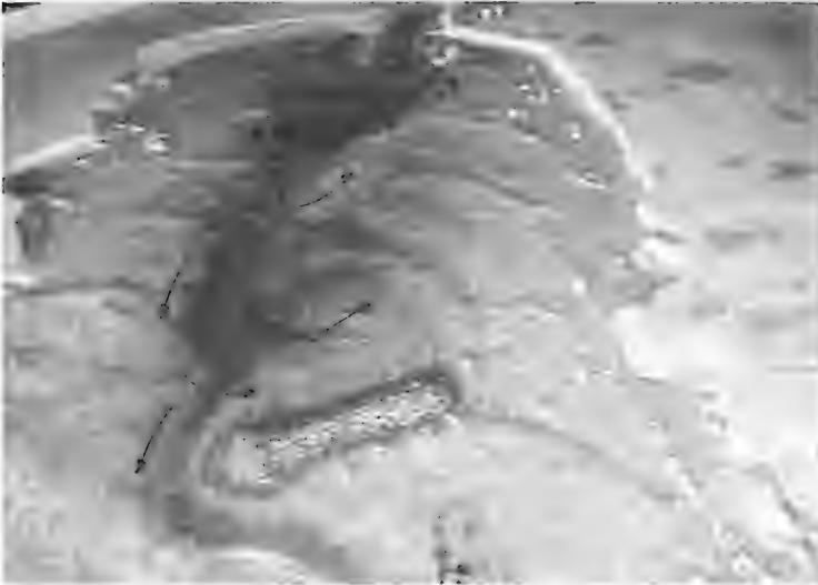
Photo 73. Riverine sediment tracer patterns for the offshore breakwater plan; 15-sec, 20-ft waves from west-northwest; swl = 0.0 ft, 33,000-cfs river discharge
