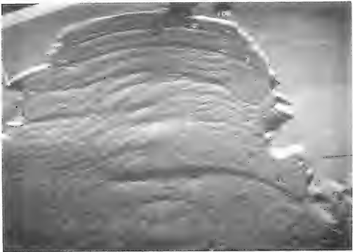
Photo 16. Typical wave patterns for existing conditions; 15-sec, 14-ft waves from west-southwest; swl = +7.0 ft
