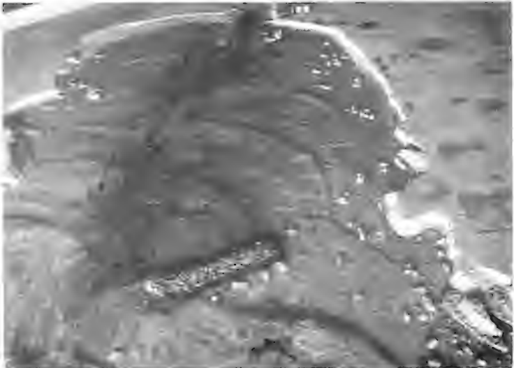
Photo 72. Riverine sediment tracer patterns for the offshore breakwater plan; 15-sec, 20-ft waves from west-northwest; swl = 0.0 ft, 27,000-cfs river discharge
