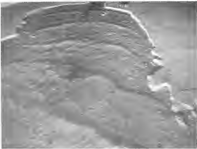
Photo 4. Typical wave patterns for existing conditions; 17-sec, 22-ft waves from northwest; swl = +7.0 ft
