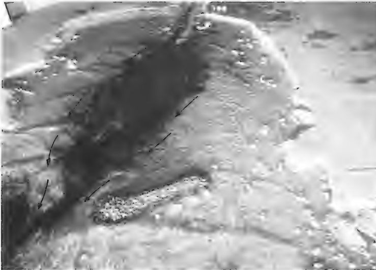
Photo 77. Riverine sediment tracer patterns for the offshore breakwater plan; 13-sec, 14-ft waves from west; swl = 0.0 ft, 33,000-cfs river discharge
