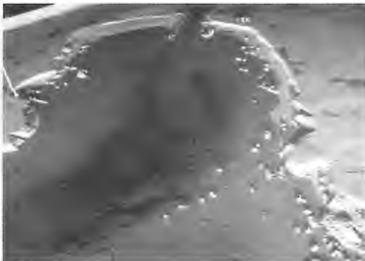
Photo 45. Riverine sediment patterns for existing conditions; 41,000-cfs river discharge
