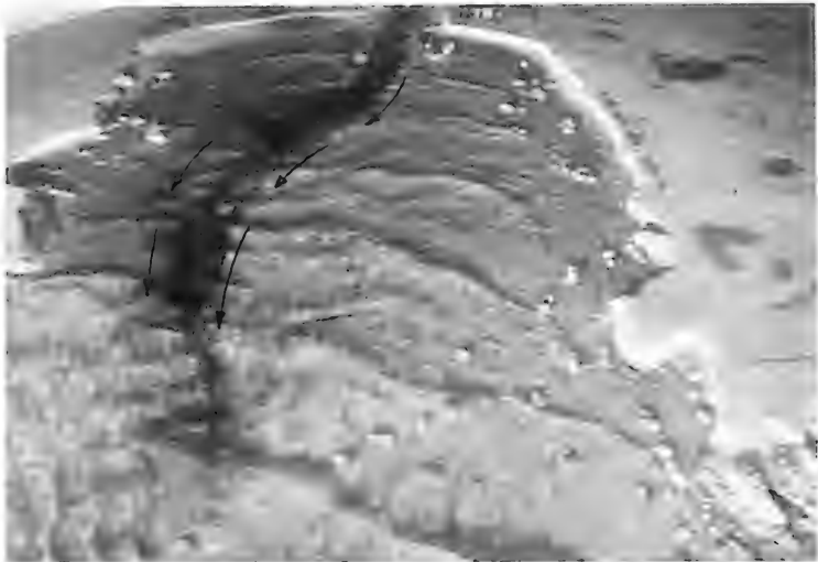
Photo 51. Riverine sediment tracer patterns for existing conditions; 13-sec, 14-ft waves from west-northwest; swl = 0.0 ft, 20,000-cfs river discharge
