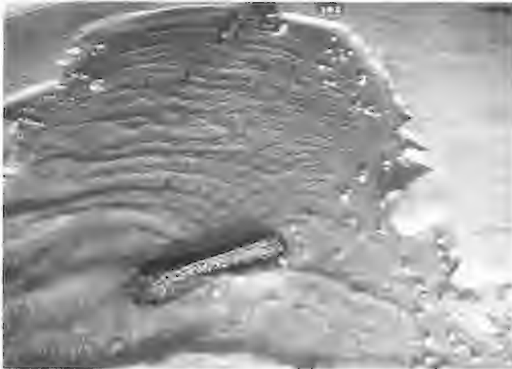
Photo 29. Typical wave patterns for the offshore breakwater plan; 11-sec, 20-ft waves from west-southwest; swl = 0.0 ft
