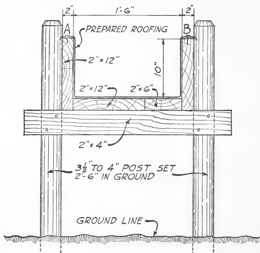
FIGURE 14.—Detail of a flume design commonly used for farm ditches. The posts are spaced 8 feet apart along the length of the flume. The prepared roofing is laid lengthwise and whatever joints are necessary are made by sealing the edges with roofing cement. The edges at a and b are securely held with roofing nails.
