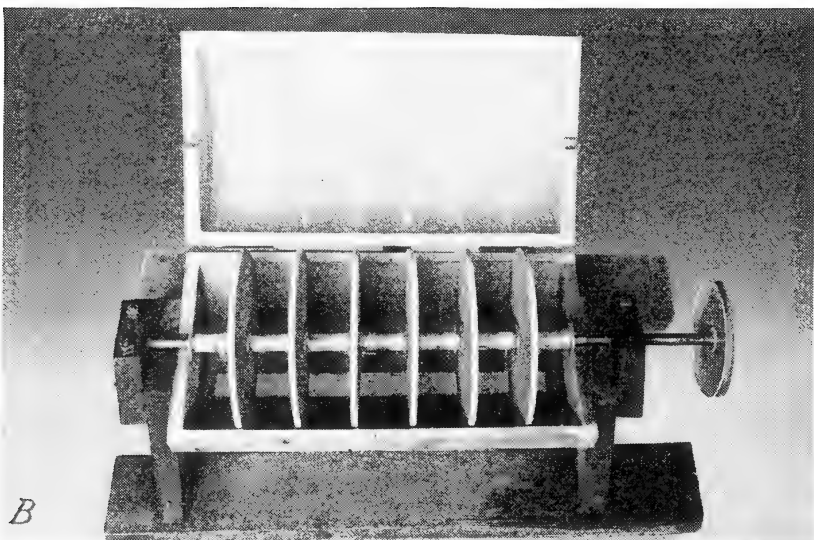
FIGURE 9.—Disk seed scarifier developed by the Lake States Forest Experiment Station. A, Exterior view; B, interior view, showing screen in bottom to allow dust to escape.
