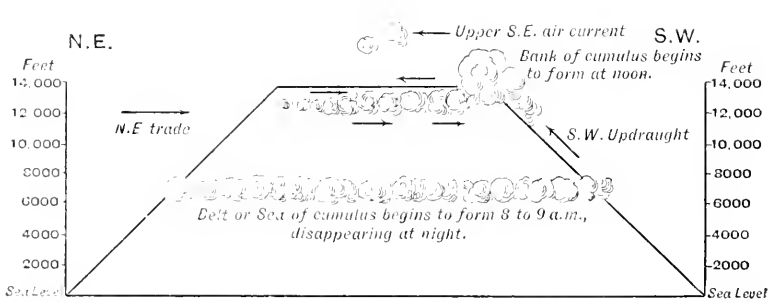
Diagram illustrating the prevailing cloud-formations of Mauna Loa during August, 1807.
