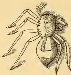
Fig. 12.— Saitis pulex . Male using all his legs to display before female.
