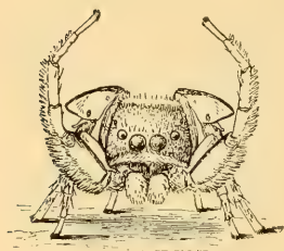
Fig. 11.—New species of Habrocestum . Male taking an attitude, before female, which displays his ornamented first legs and the apophyses on his third legs.
