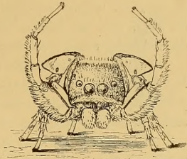
Fig. 3.—New Habrocestum, showing front view of male when approaching female (from nature).
