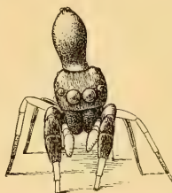
Fig. 10.— Sygnageles picata . Male displaying his iridescent first legs before female.
