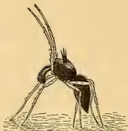
Fig. 8.— Astia vittata , var. Niger . Male striking an imposing attitude before female.
