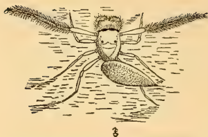
Fig. 7.— Icius mitratus . Male displaying his fringed legs before female.
