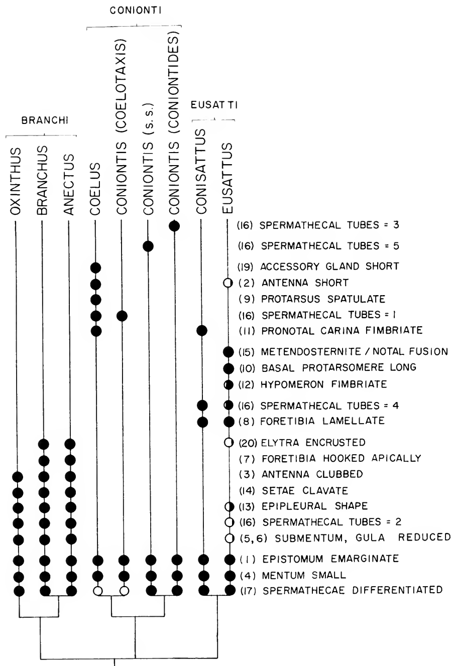
FIGURE 13. Cladogram of possible relationships among genera of Coniontiini. Numbers explained in text. Closed circles indicate universal presence of derived character states on right; partially closed circles indicate the approximate proportions (numbers of species) when both primitive and derived states are present; open circles indicate absence of information or inapplicability of character.
