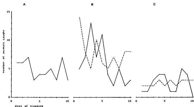
FIG. 4.—Frequency of live-trapping captures at (A) Long Pine Hills, (B) Dickinson, and (C) Cottonwood. For Dickinson and Cottonwood, broken lines show the June captures and the solid line shows the August captures.
