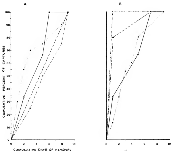
FIG. 8.—Rate of removal for the most commonly snap-trapped species in (A) the June grid and (B) the August grid at Dickinson, North Dakota. Key:
