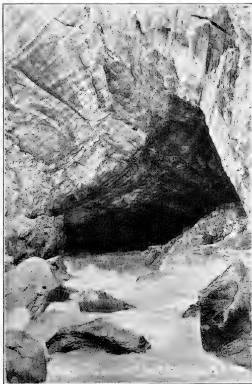
165. HOOKER RIVER PASSING UNDER MULLER GLACIER.
