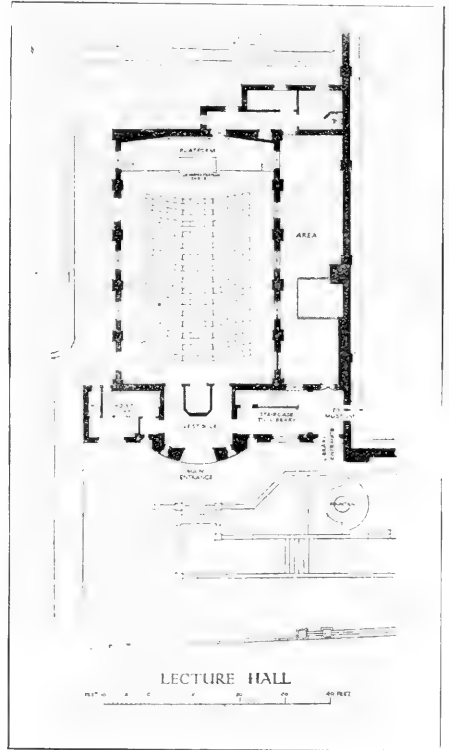
37. PLAN OF LECTURE HALL.
