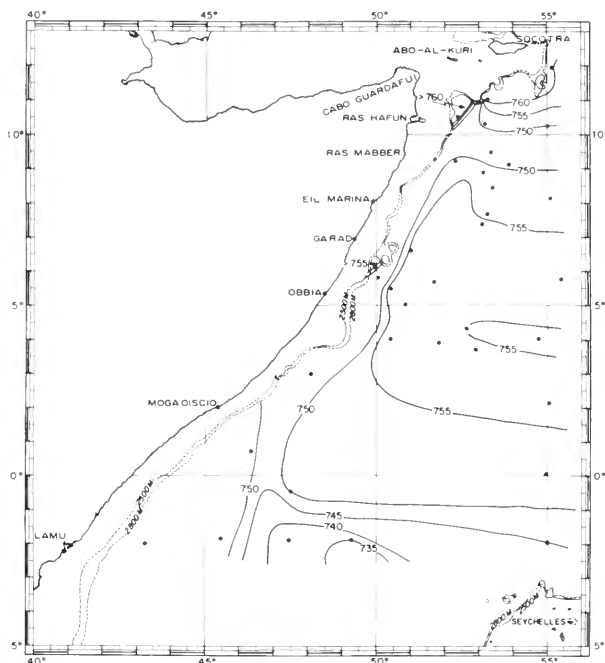
The deep current in the Somali Basin is shown on this corrected salinity chart. (34. has to be placed in front of the decimal parts). A narrow, deep flow runs along the coast and turns eastward at about 10° North, some 100-150 miles north of where the surface current turned eastward. The bottom contours of 2500-2800 meters show the boundaries for this chart.
