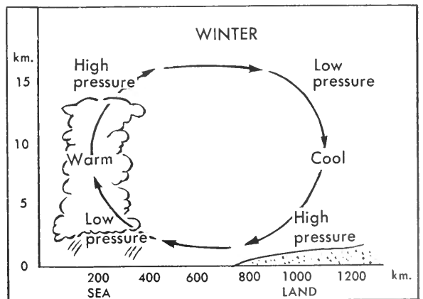
The air circulations associated with the summer and winter monsoons (after: WMO-No. 166).
