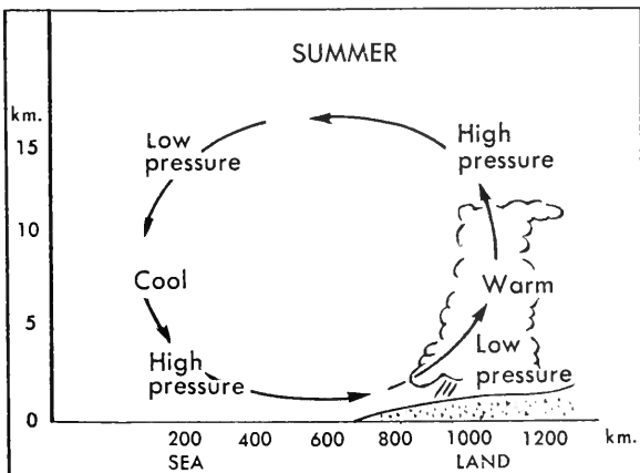
The air circulations associated with the summer and winter monsoons (after: WMO-No. 166).
