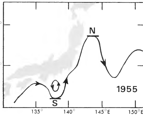
The location of the northern limit (N.) of the first meander east of Japan fluctuates over a period of 4½ to 5 years, while the location of the southern limit (S.) shows fluctuations of about eleven years due to the generation of a counterclockwise eddy off Japan.
