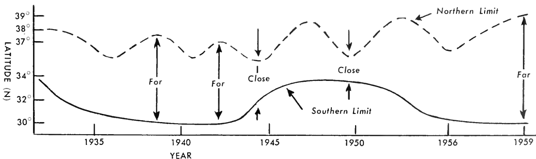
The northern limit (dotted line) and the southern limit (solid line) of the Kuroshio, as shown in the above drawings, move toward or away from each other over a period of about eleven years. The farthest separation started in 1959.
