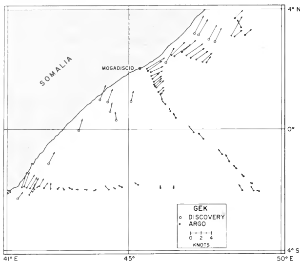
Vectors of the surface current as obtained by the GEK. The lengths of the arrows indicate the speed of the current in knots. The Somali Current is shown right up against the coast with an abrupt offshore edge. Surface speeds are about equal to those of the Gulf Stream, \pm four knots.
