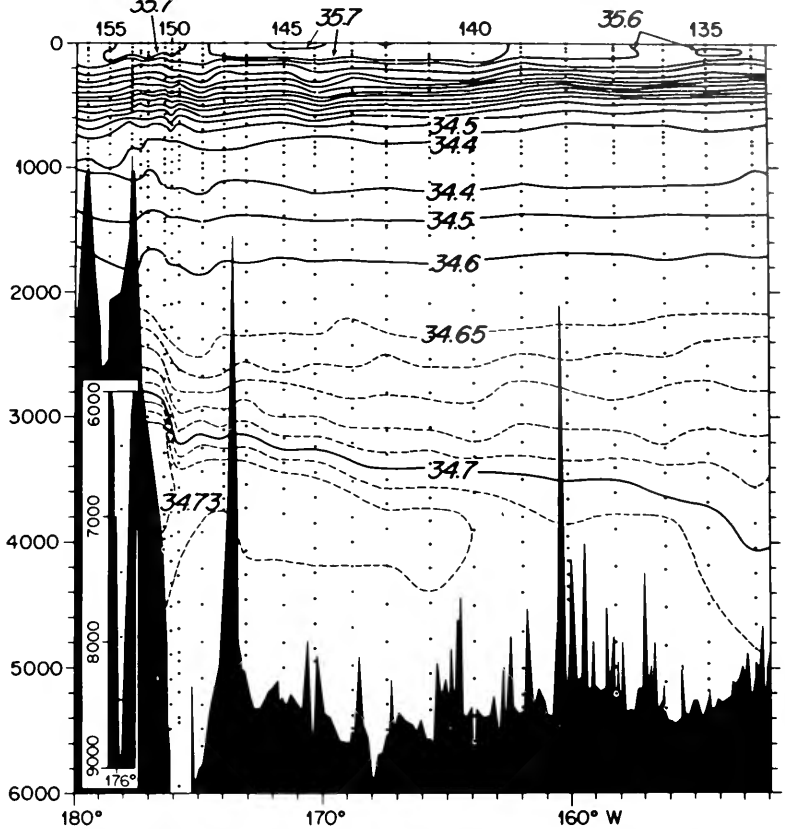
Profile of salinity in parts per thousand along Latitude 28°S in the vicinity of the western boundary of the deep South Pacific. Compare this with the corresponding temperature profile at left. For details see description below.
