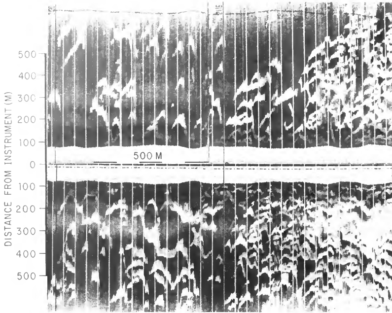
Figure 3. Side-looking sonar record of sea-floor dunes on the Carnegie Ridge off the coast of Ecuador and Peru. The boundaries between light and dark areas near the center of the record are the sea-floor profile directly beneath the instrument; the lower and upper parts of the record represent the sea floor to the left and right of the instrument track. (Courtesy Peter Lonsdale and Fred N. Spiess, Scripps Institution of Oceanography)
