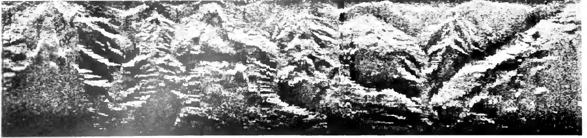
Figure 10. A side-scan sonar (4 kilohertz) inspection of the continental slope from the shelf edge south of the English Channel into the Bay of Biscay. Bright areas are shadows; dark areas have been ensonified. Note the marked diagonal channels and the intricate tributary system feeding the main diagonal canyons. The scene is approximately 12 kilometers from top to bottom and 48 kilometers long. (Courtesy Institute of Oceanographic Sciences, Britain)
