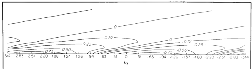
Figure 3. Contours of constant sea level elevation calculated from model, with idealizations as illustrated in Figure 2. A full “wave” of the wind is shown from ky = -\pi to +\pi . At y=0 , the wind blows with maximum strength to the left. The y axis is the coastline. Significant elevations are confined to a narrow nearshore band.
