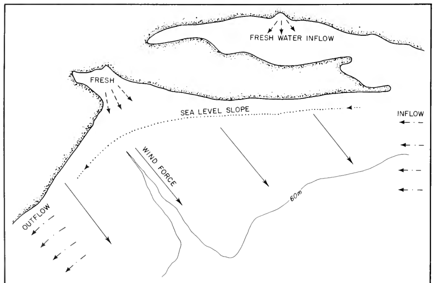
Figure 1. Portions of the coastline of the Mid-Atlantic Bight near New York, showing forces driving the circulation over a typical ocean continental shelf. These include the wind force, freshwater inflow, and an alongshore sea-level slope. Inflow and outflow across open boundaries of a chosen shelf region complicate the mathematical modelling of these phenomena.
