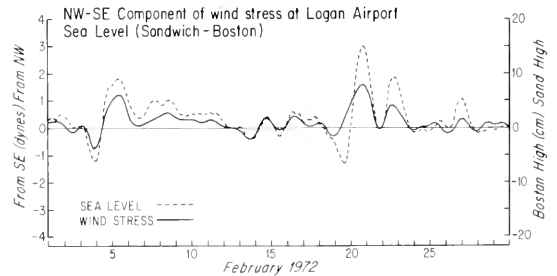
Figure 6. Sea-level difference between Sandwich (on Cape Cod) and Boston, compared with component of wind force that points alongshore on this region of coast. (From Ph.D. thesis of Bradford Butman)
