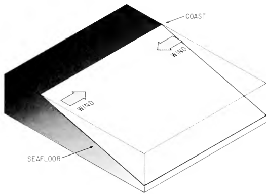
Figure 2. Idealized straight coast and inclined plane beach, subject to variable longshore wind.
