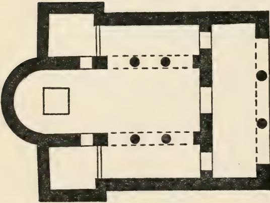
PLAN OF CHURCH AT SILCHESTER AND CONJECTURAL RESTORATION (15 feet to 1 inch)
