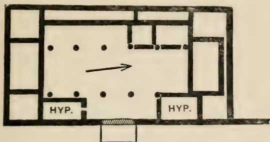
HOUSE AT CLANVILLE (40 FEET TO \frac{1}{4} INCH)
