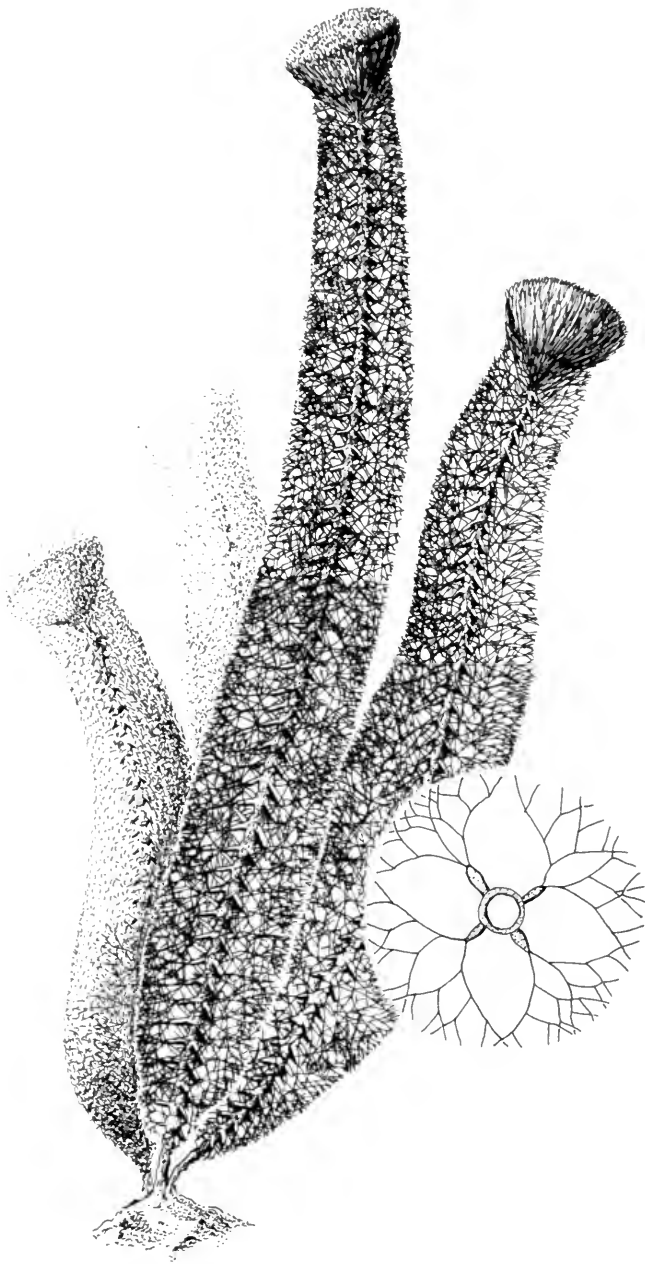
FIG. 2. Reconstruction of Archaeobatophora typa n.g. and sp. The holdfast is conjectural. Inset: cross-section through thallus.
