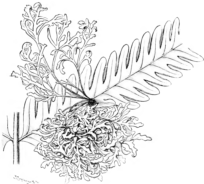
FIG. 103. Preris quadriaurita . 'Witches' broom' upon a leaf pinna. Its leaves differ in form from the normal ones of the fern. The malformation is induced by the attack of the parasitic fungus Taphrina Laurencia . After Giesenhagen.
