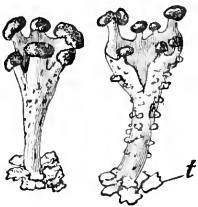
FIG. 31. Cladonia coccifera . A cup-like podetium bearing marginal stalked apothecia rises from the horizontal thallus. (Lehrb.)
