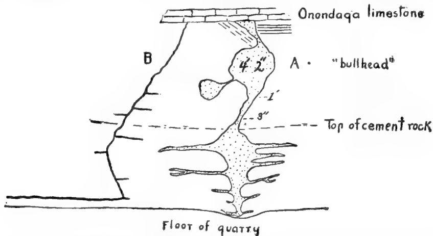
Diagram showing the largest of the sand dikes (A) in the quarries of the Buffalo cement co., at Buffalo N. Y. The floor of the quarry is the lowest layer used for burning cement and while the dike seems to enter this stratum it does not penetrate it. The figure shows the irregular character of the fissure walls, and the lateral apophyses in the lower part which are essentially parallel to the bedding. At the top is a slight displacement of the "bull-head" or Manlius waterlime on one side of the dike. B shows a second dike, the filling of a very narrow fissure. Others are evident elsewhere in this quarry. The Onondaga limestone lies horizontally over them all and is not penetrated by them.
