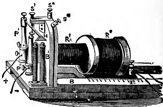
FIG. 94.—Induction Apparatus of Du Bois-Reymond. R' . Primary, R'' . Secondary spiral; B . Board on which R'' moves; I . Scale; + -. Wires from battery; P , P' . Pillars; H . Neef's hammer; E . Electro-magnet; S . Binding screw touching the steel spring ( H ); S' , and S'' . Binding screws to which are attached wires when Neef's hammer is not required.
