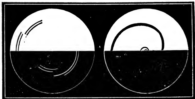
FIGS. 283 and 284.—Modifications of Discs for Benham's Spectrum Top ( Hurst ).
