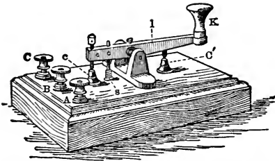
FIG. 87.—Morse Key. The connections are concealed below, but are B to l , A to c , C to C '.
