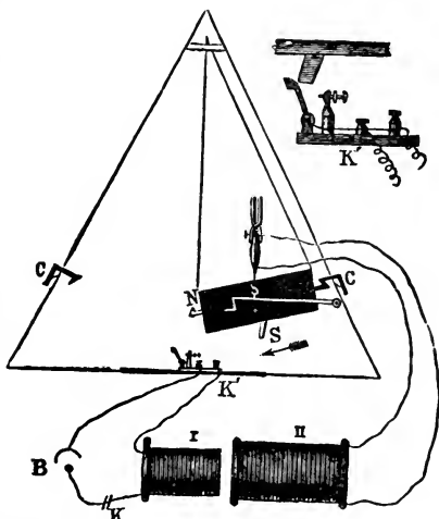
FIG. 125.—Scheme of the Arrangement of the Pendulum. B . Battery; I . Primary, II . Secondary spiral of the induction machine; S . Tooth; K' . Key; C, C . Catches; K' in the corner, Scheme of K' ; K . Key in primary circuit. It is well to have a short-circuiting key in the secondary circuit.
