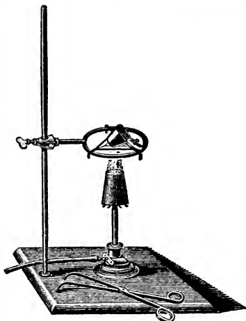
FIG. 19.—Method of Incinerating a Deposit to Obtain the Ash.
