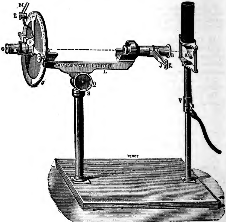
FIG 12.—Laurent's Half-Shadow Polarimeter.
