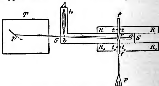
FIG. 140.—Scheme of Blix's Myograph. S, S Slider; R, R and R', R' Guides for slider; a, b Lever; A for muscle; P , Weight; r , Collar; t, t and t_1, t_1 Guides for collar carrying weight; p , Recording point.
