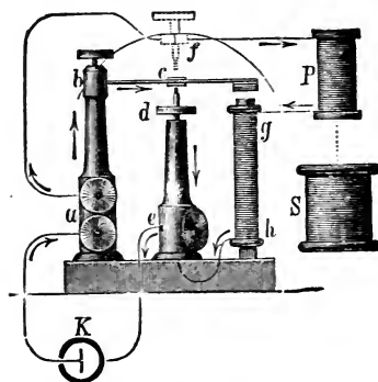
FIG. 102. — Helmholtz's Modification of Neef's Hammer. As long as c is not in contact with d , g h remains magnetic; thus c is attracted to d , and a secondary circuit, a, b, c, d, e , is formed; c then springs back again, and thus the process goes on. A new wire is introduced to connect a with f . K. Battery.
