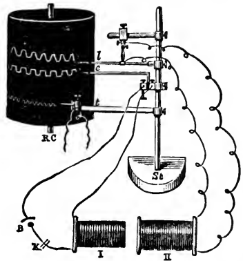
FIG. 128.—Arrangement for Estimating the Time-Relations of a Single Muscular Contraction. B. Battery; K. Key in primary circuit; I. Primary, II. Secondary coil, without a short-circuiting key; L. Muscle-lever; e. Electro-magnet in primary circuit; t. Electric signal; St. Support; RC. Revolving cylinder. Introduce a short-circuiting key into the secondary circuit.
