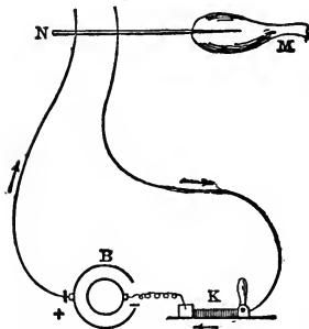
FIG. 85.—Scheme of Du Bois Key. B. Battery; K. Key; N. Nerve; M. Muscle.
