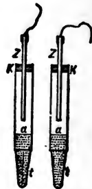
FIG. 157.—Non-Polarisable Electrodes. Z. Zincs; K. Cork; a. Zinc sulphate solution; t, t. Clay points.
