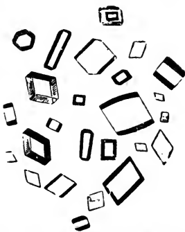
FIG. 61.—Crystals of Oxalate of Urea from Urine.
