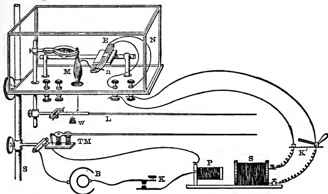
FIG. 116.—Moist Chamber. N. Glass shade; E. Electrodes; L. Lever; W. Weight; TM. Time-marker; other letters as in previous figures.
