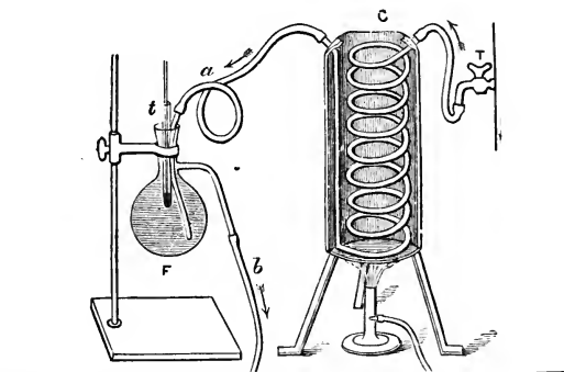
FIG. 2.—Apparatus of Halliburton for Fractional Heat Coagulation of Proteids. T. Tap for Water; C. Copper vessel with spiral tube; a. Inlet, and b. Outlet-tube to the flask; t. Test tube, with fluid and thermometer.
