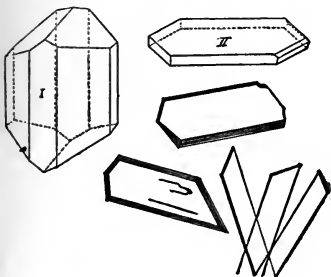
FIG. 7.—Crystals of Maltose.
