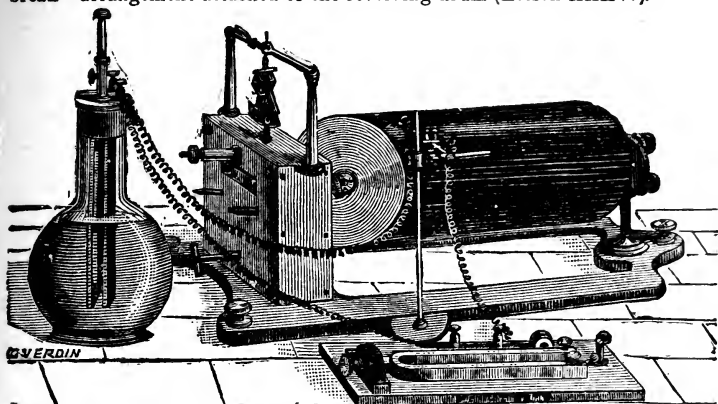
FIG. 131.—Chronograph arranged to Write on a Horizontal Cylinder, as made by Verdin.
