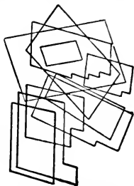
FIG. 45.—Crystals of Cholesterin.
