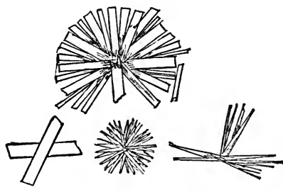
FIG. 8.—Crystals of Phenyl-Maltosazone, \times 120 .
