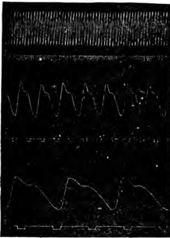
FIG. 189.—Shows how Heart Curve varies with rate of Drum. In 1, 2, 3, T' = time in seconds. Gaskell's Lever.
