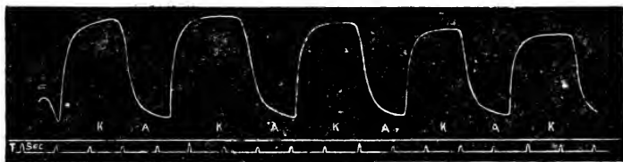
FIG. 170.—Tracing showing effect of Anode and Kathode on Excitability of Nerve, the latter stimulated with repeated shocks. T. Time in seconds.
