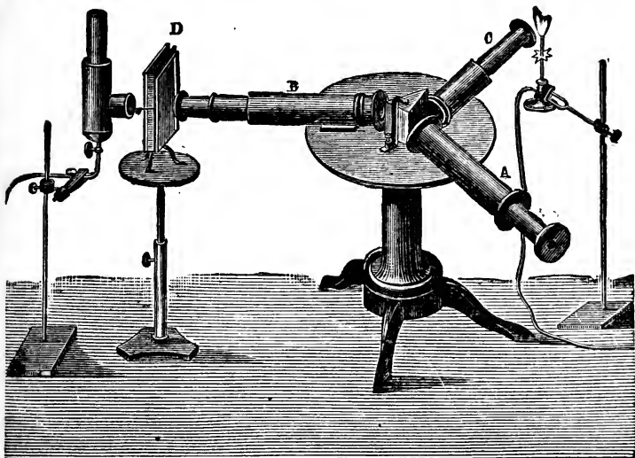
FIG. 31.—Arrangement of the Spectroscope for Determining Wave-Lengths. A. Telescope; B. Collimator tube; C. Scale tube; D. Hæmatinometer.
