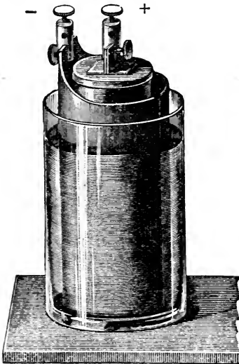
FIG. 81.—Large Grove's Element.
