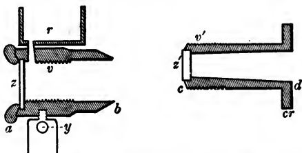
FIG. 38.—Showing how cd fits into ab . zz . Plates of glass closing the ends of ab and cd ; other letters as in fig. 37.
