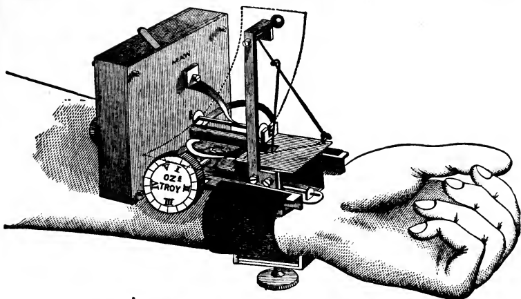
FIG. 216.—Dudgeon's Sphygmograph.
