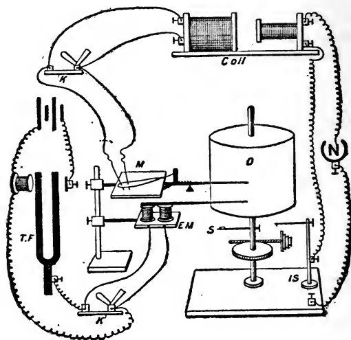
FIG. 120.—Arrangement for analysis of Muscle-Curve by means of Crank-Myograph (M) with "Automatic Break" Arrangement in Primary Circuit. S. Striker on axis of D cylinder; P.C. Primary, and S.C. Secondary circuits; T.C. Time-circuit with E.M. Electro-magnet; I.S. Insulated support in P.C.
