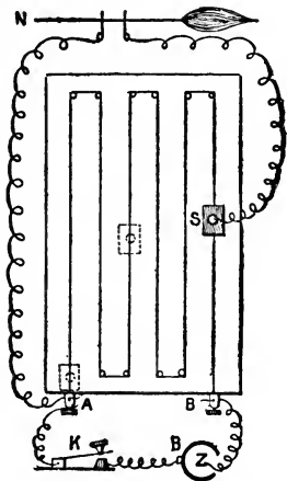
FIG. 92.—Simple Rheochord as used in Oxford. B. Battery; K. Spring-Key; A. B. Terminals of Rheochord Wire; S. Slider; N. Nerve.
