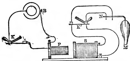
FIG. 109.—Scheme for Single Induction Shocks. B. Battery; K, K'. Keys; P. Primary, and S. Secondary coil of the induction machine; N. Nerve; M. Muscle.
