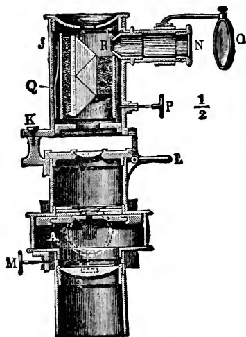
FIG. 39.—Zeiss's Microspectroscope after Albe.
