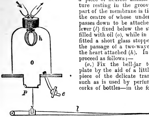
FIG. 205.—Scheme of Roy's Tonometer.
