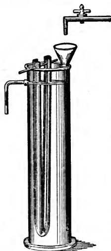
FIG. 43.—Kühne's Dialyser. A parchment tube, such as is used for sausages, is suspended in a vessel through which water is kept continually flowing.
