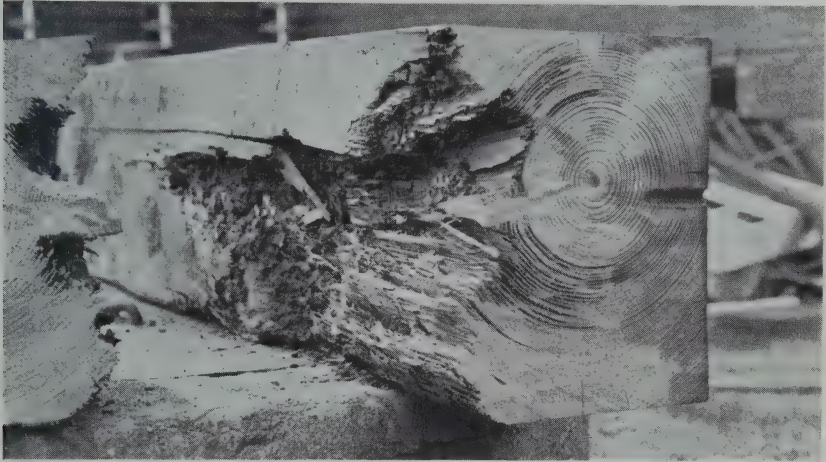
Fig. 9.—Termite injury to the frame of a large school building. In this case the entire sill had been honeycombed and largely destroyed by termites, which had built their tunnels in it.
