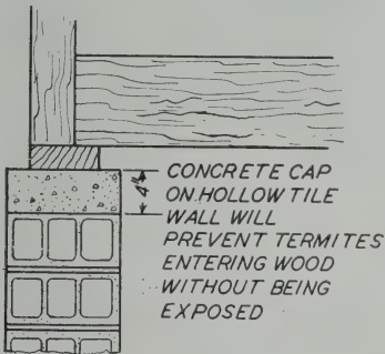
Fig. 11.—Passage of termites through or between hollow unit masonry foundation into wood sills above may be prevented by capping such a wall with four inches of good concrete. The termites may build tubes over this concrete, but, when they do this, their presence is easily detected.
