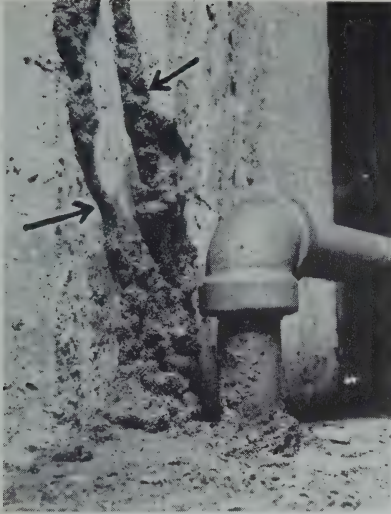
Fig. 4.—Very large termite tubes extending through a poorly constructed concrete floor over a concrete basement wall.
