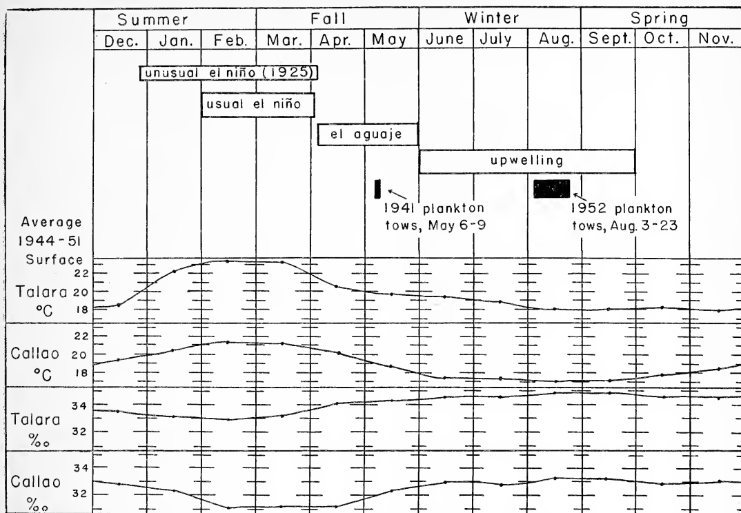
FIG. 14. The relationship of the 1941 and 1952 plankton samples to the physical environment off Peru. The extent in time of El Niño, El Aguaje, and upwelling are taken from Sverdrup, Johnson, and Fleming, 1942. The average surface temperature in degrees centigrade and surface salinity in 0/00 are based on Coast and Geodetic Survey publications 280 and 281. The increase in temperature and concurrent decrease in salinity during the months of January through April are conspicuous.
