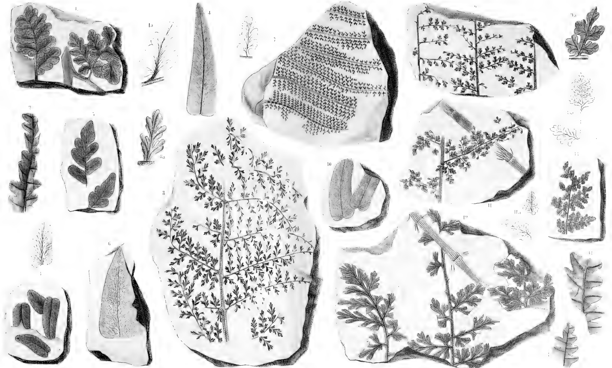
1 Sphenopteris Schillingsii Andrae. — 2 14 15 Meliopteris irregularis v. Roehl. — 3 10 Neuropteris flexuosa Sternbq. — 4 Neuropteris acutifolia Brong. — 5 Odontopteris neuropteroides F. A. Roemer. — 6 Dictyopteris cordata F. A. Roemer. — 7 Sphenopteris coralloides v. Gutb. — 8 Sphenopteris elegans Sternbq. — 9 Sphenopteris distans Sternbq. — 11 13. Sphenopteris formosa v. Gutb. — 12 Hymenophyllites furcatus Brong.
