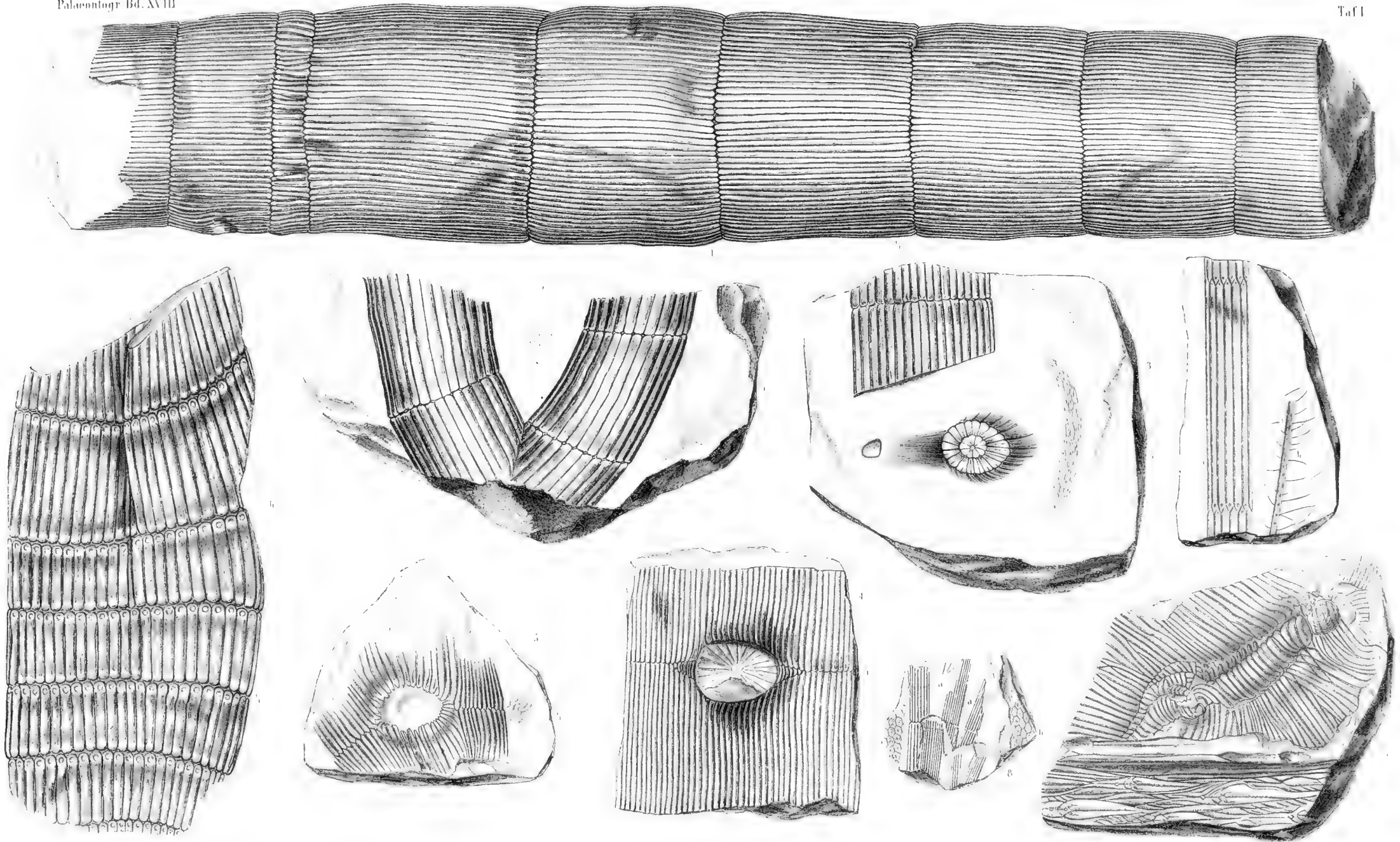
1 Calamites varians Sternb. 2, 5 Calamites cañaeformis Schloth. 3, 4 Calamites ramosus Artis. 6 Calamites Suckowii Brong. 7a Calamites Roemeri Goep. b Pinularia capitata Lindl. 8 a-jüngere Stämme v. Calamites cañaeformis Schloth. b Sigillaria minima Brong. 9 Alt. Ansatz eines Calamiten nebst Lepidodendron aculeatum Sternbq.
