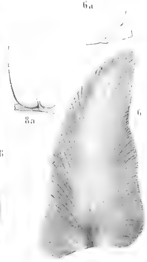
1 Frucht von Lepidophloos farcinum Sternbg — 2 Hymenophyllites furcatus Bryn — 3 Sphenopteris Hoeninghausii Bry — 4 Althopteris Mantelli Goepf — 5 Pecopteris subnervosa Roemer — 6 Neuropteris cordata Bry 7 Althopteris marginata Goepf — 8 Neuropteris plicata Sternbg
