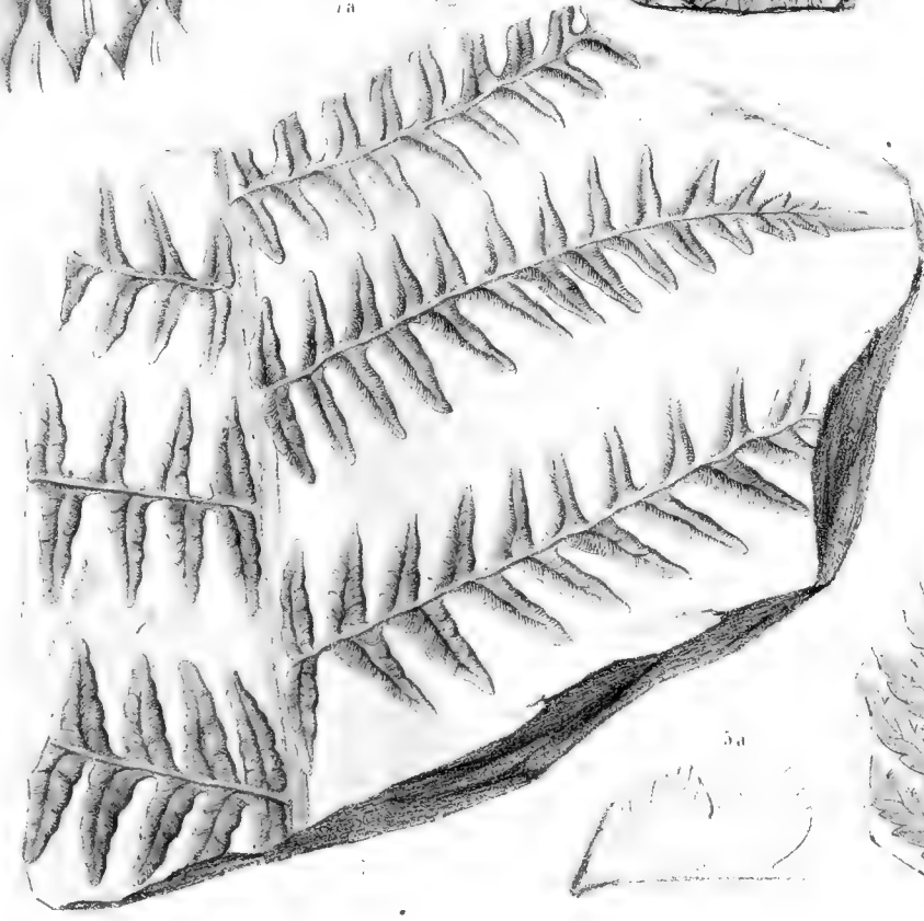
1 Frucht von Lepidophloos farcinum Sternbg — 2 Hymenophyllites furcatus Bryn — 3 Sphenopteris Hoeninghausii Bry — 4 Althopteris Mantelli Goepf — 5 Pecopteris subnervosa Roemer — 6 Neuropteris cordata Bry 7 Althopteris marginata Goepf — 8 Neuropteris plicata Sternbg
