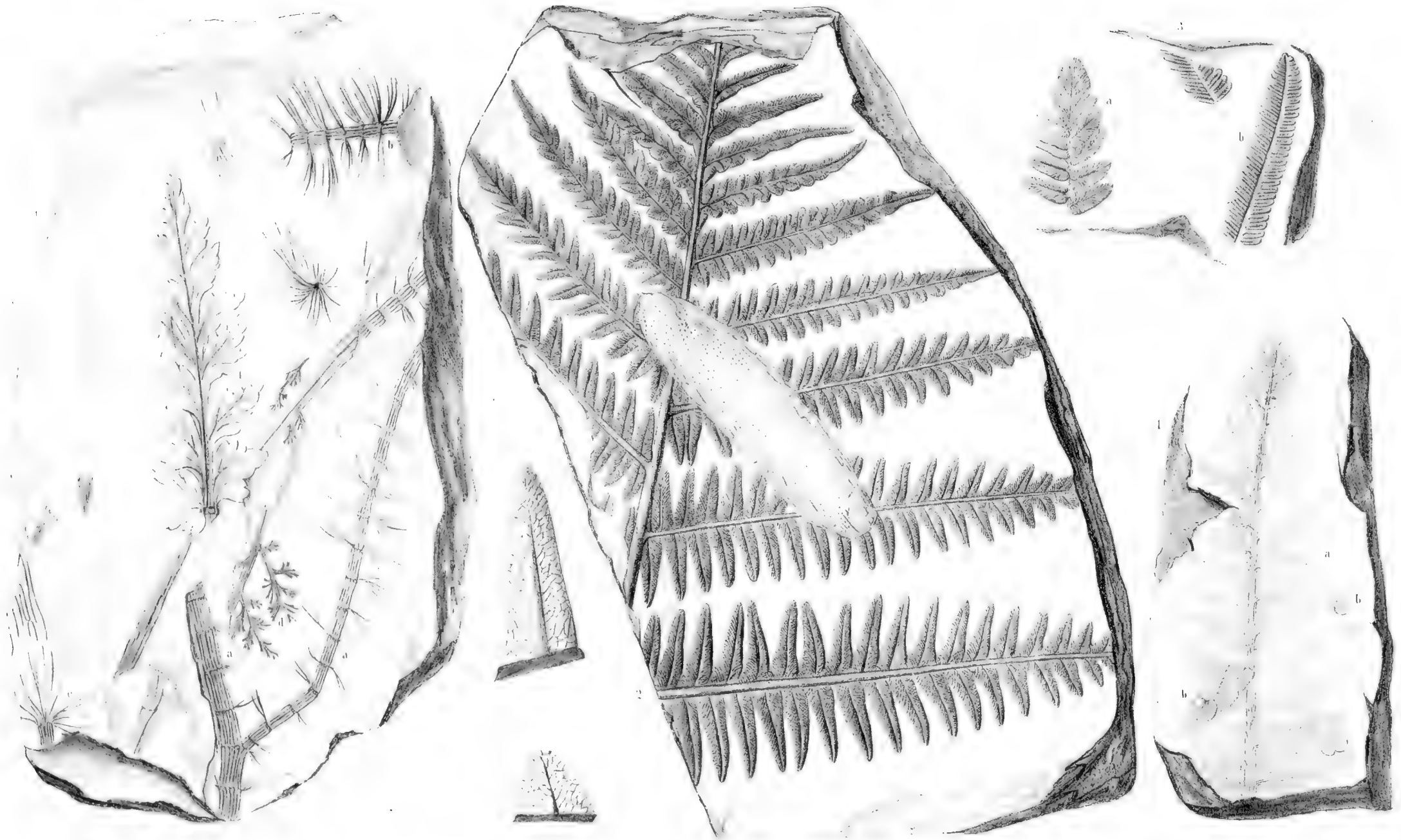
1a,b Volkmannia gracilis Sternbg., c Asterophyllites longifolia Sternbg., d Hymenophyllites fureatus Brq., e Sphenopteris macilenta Lindl et Hutt. — 2 Lonchopteris Roehlii Andrae — 3 a, Neuropteris flexuosa Sternbg., b Cyathites Candolleanus Goeppl. — 4 a Neuropteris acutifolia Brq., b Neuropteris rotundifolia v Gutb. —
