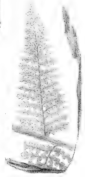
1 Frucht von Lepidophloos farcinum Sternbg — 2 Hymenophyllites furcatus Bryn — 3 Sphenopteris Hoeninghausii Bry — 4 Althopteris Mantelli Goepf — 5 Pecopteris subnervosa Roemer — 6 Neuropteris cordata Bry 7 Althopteris marginata Goepf — 8 Neuropteris plicata Sternbg
