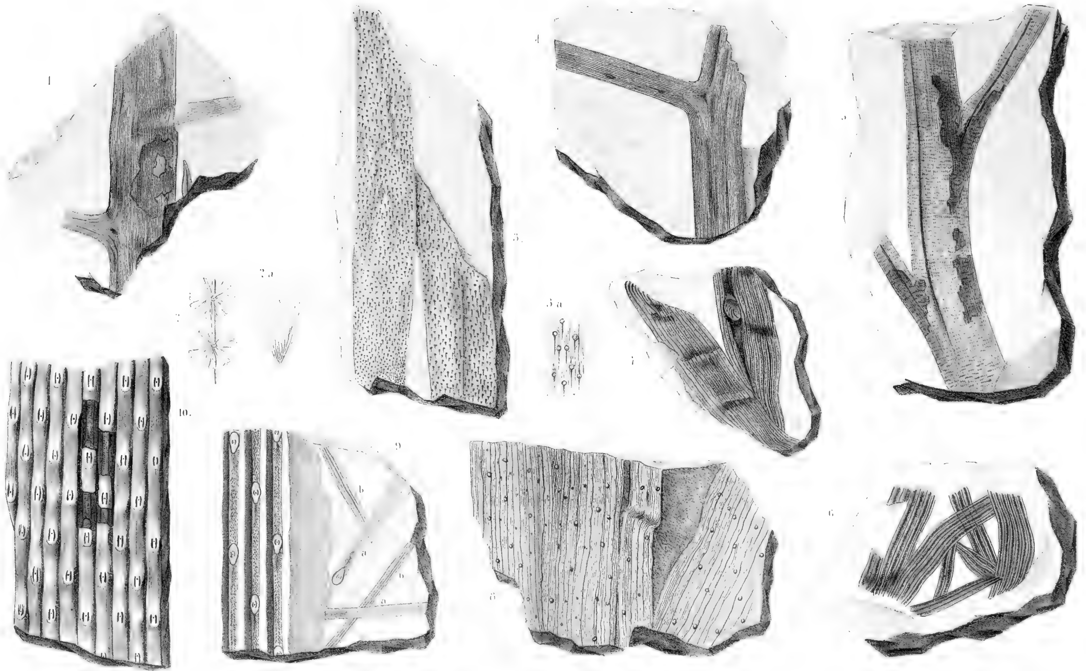
1. Noeggerathia tenuistriata Goeppl. — 2. Sphenophyllum emarginatum Brongniart var. Brongniartianum Coen et J.J. K-x. — 3. Strunk von Cyatheetes arborescens Goeppl. — 4. Strunk von Sphenopteris elegans Brong. — 5. Equisetites zeaeformis Schloth. — 6. Noeggerathia Dückeriana v. Roehl. — 7. Sigillaria subrotunda Brong. — 8. Sigillaria ocellata Sternbg. var.
