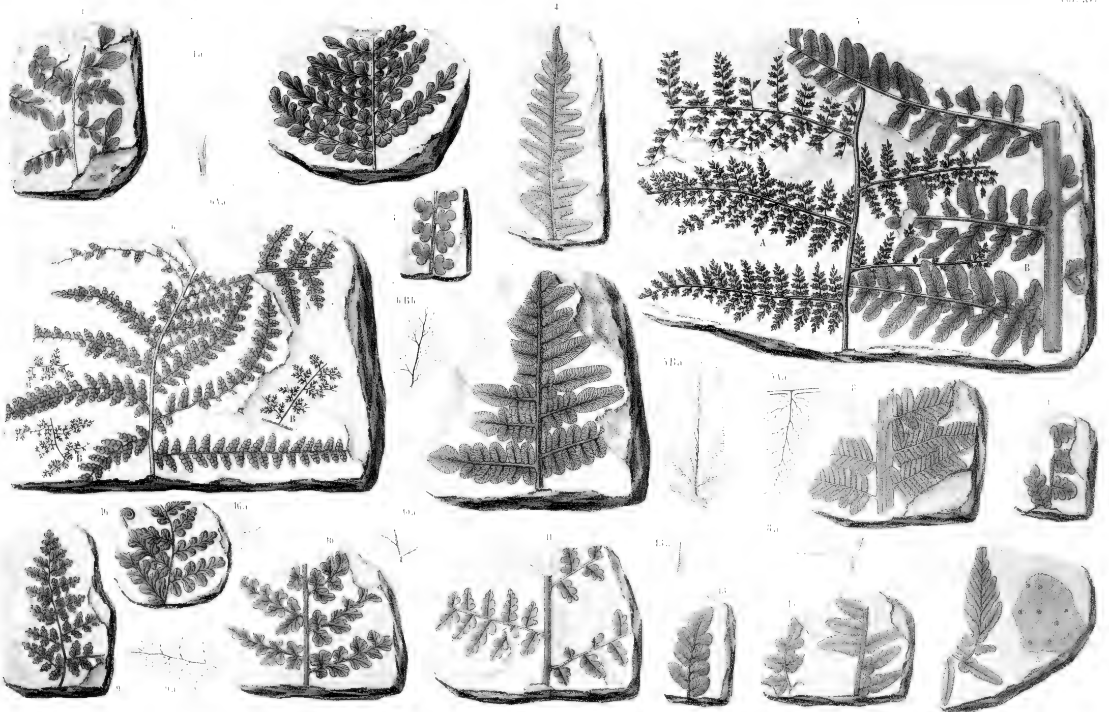
1 Cyclopteris oblongifolia Goepp var. sessilis v. Roehl. — 2 Sphenopteris irregularis Sternb. — 3 Sphenopteris trifoliolata Arls. — 4 Lonchopteris rugosa Brong. — 5 A Sphenopteris Bromii v. Gutb. — 5 B Xenopteris heterophylla Sternb. — 6 A Sphenopteris stipulata v. Gutb. — 6 B Trichomanoides delicatulus Brong. — 7 Xenopteris imbricata Goepp var. densinervis v. Roehl. — 9 Sphenopteris formosa v. Gutb. — 10 I Sphenopteris obtusiloba Brong. — 10 II Sphenopteris obtusiloba Brong. — 12 — 13 Odonopteris obtusiloba Naum. — 14 A mit Sporobis carbonarius Daws. — 16 Sphenopteris trifoliolata Arls.
