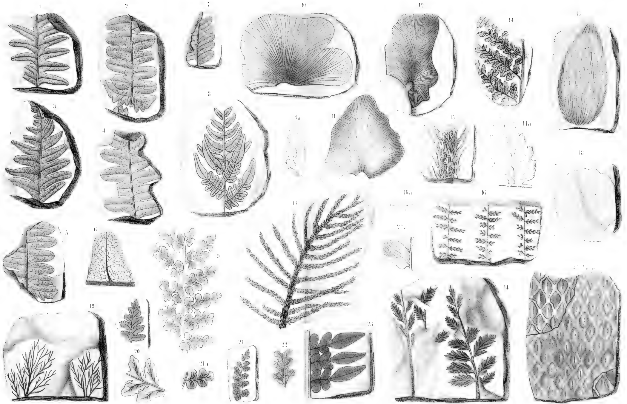
1-7 Lonchopteris rugosa Brong. - 8 Dietyopteris Hoffmanni F.A. Roemer. - 9 Sphenopteris obtusiloba Brong. - 10 Cyclopteris trichomanoides Brong. - 11 Cyclopteris varians (Curt.) - 12 Cyclopteris obliqua Brong. - 13 Lycopodites Brownii Sternbg. - 14 Sphenopteris cristata Sternbg. - 15 Lepidodendron obovatum Sternbg. - 16 Sphenopteris grypophylla Goepf. - 17 Lepidostrobus variabilis Lindl. et Hutt. - 18 Cyclopteris peltata F.A. Roemer. - 19 Hymenophyllites dissectus Brong. - 20 Pecopteris decurrens F.A. Roemer. - 21 Sphenopteris pentaphylla F.A. Roemer. - 22 Odontopteris connata F.A. Roemer. - 23 Odontopteris oblongifolia F.A. Roemer. - 24 Sphenopteris fascicularis F.A. Roemer. - 25 Lepidodendron Mielecki Goepf.
