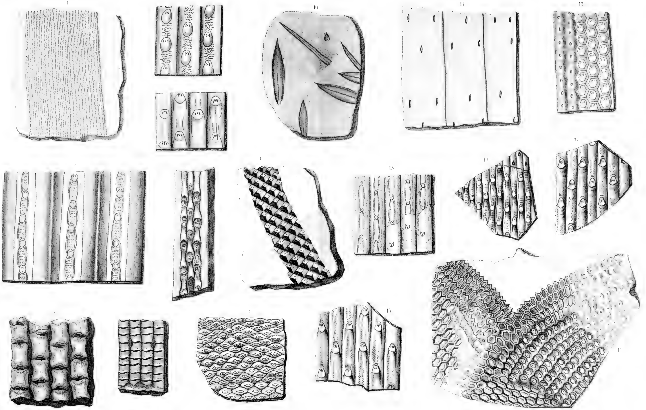
1. Sigillaria Ludwigi v. Roehl. 2. Sigillaria Polleriana Brong. 3. Sigillaria elliptica Brong. 4. Sigillaria orbicularis Brong. 5. Sigillaria diploderma Corda. 6. Sigillaria elegans Brong. 7. Sigillaria ocellata Brong. 8-9. Lepidophloem loricatum Sternbg. 10. Lepidophloem cancellatum Brong. 10 g. Cardiocarpon Gutbieri Geinitz. 11. Sigillaria distans Geinitz. 12. Sigillaria Knorri Brong. 13. Sigillaria cyclostigma Goldenbg. 14-16. Sigillaria sentellata Brong. 17. Sigillaria elegans Brong.
