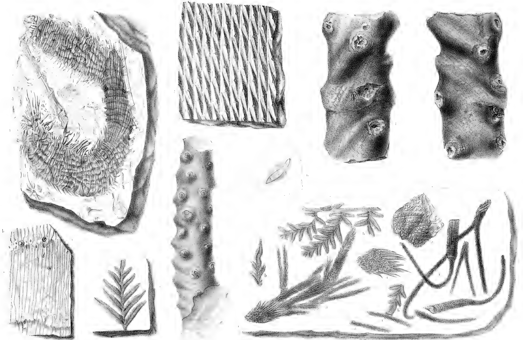
1 Huttonia carinata Germar — 2 Lepidodendron rimosum Sternbg — 3 Calamites canasiformis Schloth — 4 5 6 Halonia tuberculata Brong — 7 Halonia Munsteriana Goepf — 8 9 b Melthopteris Serlii Brong — 9 Lepidodendron dilatatum Lindl et Hutt
