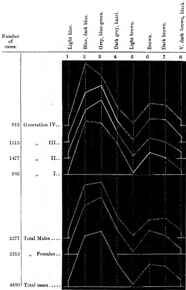
Fig. 9. Percentages of Eye-Colour in Successive Generations.
