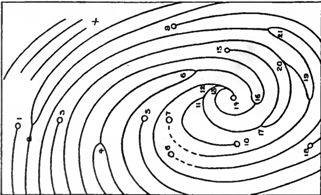
Corresponding numbers in upper and lower prints indicate persistence of minutiae .
