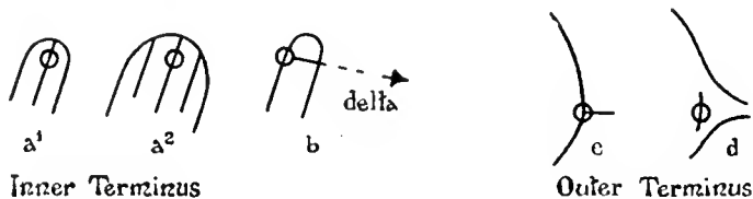
Fig. 34. Inner and Outer Termini for Ridge Counting.
