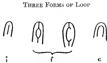
Fig. 38. Classification of Cores of Loops.
