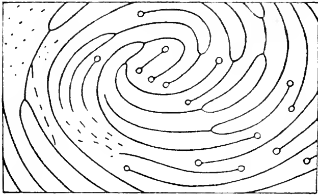
Superposition of Central Lines of Ridges on enlarged Finger-Prints. i.e. Plate XXI overprinted on Plate XX, reproduced in fainter ink.
