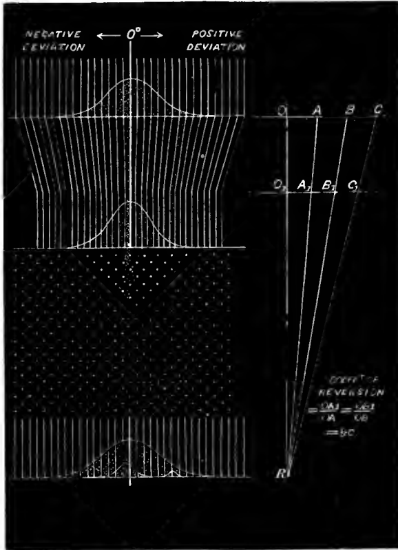
Fig. 2. Galton's Quincunx illustrating the nature of Regression.
