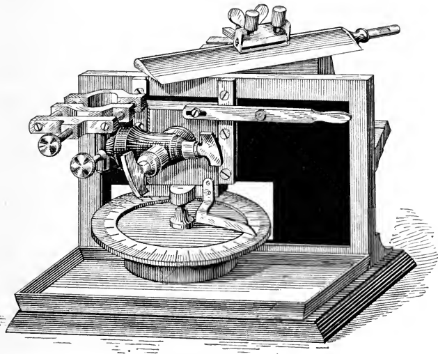
FIG. 27.—Schanze microtome.
