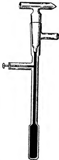
FIG. 47.—Reichert's gas-regulator.
