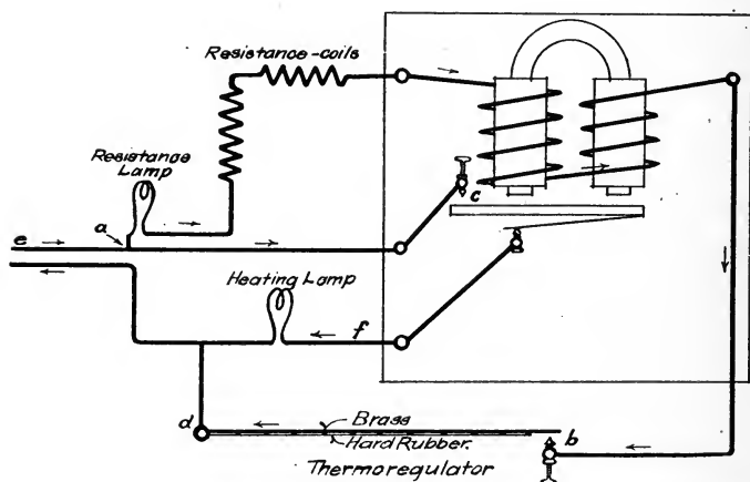
FIG. 51.—Diagram of electric regulator for low-temperature incubator.
