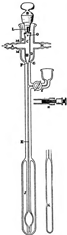
FIG. 48.—Mac Neal gas-regulator.
