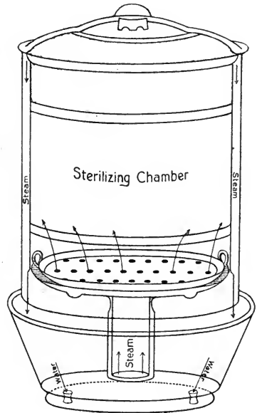
FIG. 35.—Diagram of the Arnold steam sterilizer.
