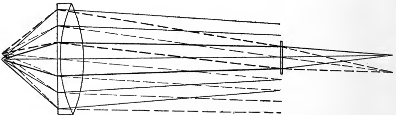
FIG. 5.—Image formation by two lenses in series, with magnification of three diameters. Note that the opening angle of the beam is three times as large as the closing angle.
