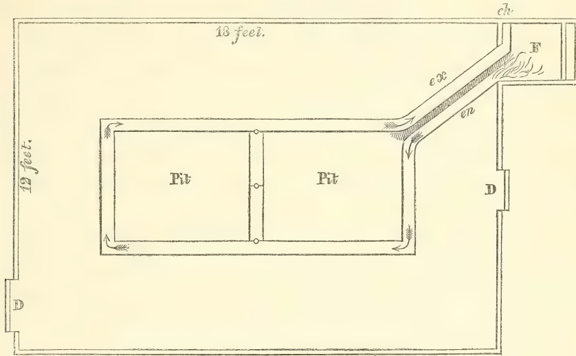
GROUND PLAN.
