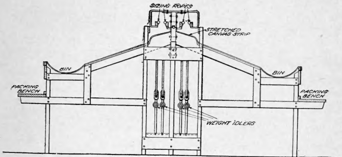
FIG. 3.—Cross-section view.
