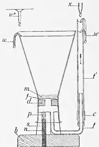
FIG. 4. Larger washing apparatus made from a flask. Diaphragm of cork or rubber, d ; filter paper, f ; material, m ; plug, p ; supporting rod, n ; rubber stopper with two holes, s ; glass tubes, t and t' ; rubber connection, c ; base, b ; filter paper wicks, w and w' ; supply of water, x ; wick in front view of lip, w'' \times \frac{3}{4} .
