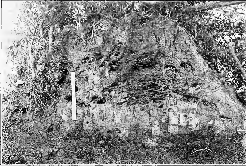
Fig. 1. Vertical section through the center of a termite nest.
