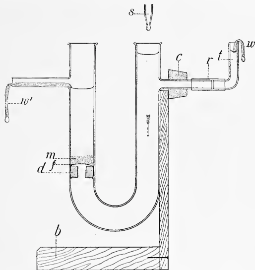
FIG. 3. Smaller washing apparatus made from a calcium chlorid tube. Diaphragm of cork or rubber, d ; filter paper, f ; material, m ; filter paper wicks, w , and w' ; glass tube, t ; rubber connection, r ; cork hanger, c ; supply of water, s ; base of stand, b . \times \frac{1}{3} .
