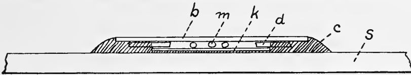
FIG. 2. Sectional view of permanent mount. Slide, s ; larger cover, b ; smaller cover, k ; glass rodlets, d ; balsam, c ; material, m . About 2\frac{1}{2} times natural size.
