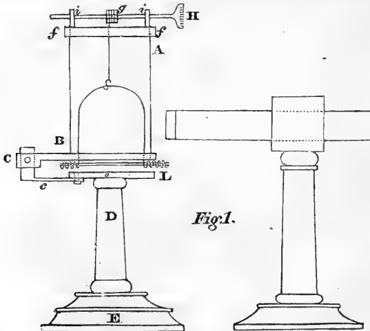
Fig. 1. A cylindrical glass tube supported by the arm Cc of
