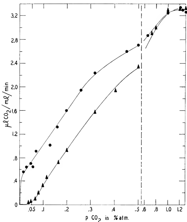
Fig. 37D.2. Adaptation to bicarbonate (after Gaffron and Rosenberg 1953). Scenedesmus in 2 \times 10^{-3} M bicarbonate. After incubation in 50% \text{CO}_2 , cells were transferred into 4% \text{CO}_2 and illuminated until all \text{CO}_2 was consumed (lower curve). After 1 hour, 4% \text{CO}_2 was added and cells illuminated until all \text{CO}_2 was again used up (upper curve).
