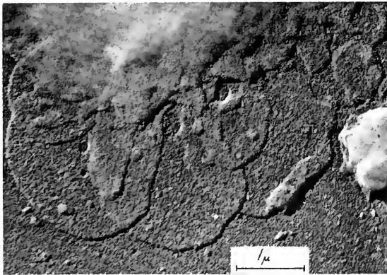
Fig. 37A.9. Electron micrographs showing the not-folded blebs that surrounded a maize chloroplast isolated in distilled water and then dried (after Vatter 1952). Compare with fig. 37A.5.
