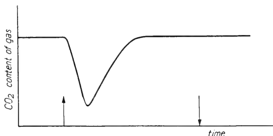
Fig. 33.13E. \text{CO}_2 uptake by Sciadopitys needles at 0^\circ \text{C} . (photosynthesis suspended) (after van der Veen 1949 1 ). Uptake normal, release in dark absent (or delayed). Diaferometer record.
