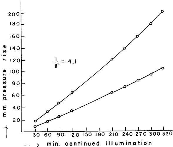
Fig. 37D.27A. Oxygen liberation by a dilute Chlorella suspension (initial absorption, 6.2%) (after Warburg et al. 1953). Upper curve: smaller vessel; lower curve: larger vessel. \lambda 546 \text{ m}\mu , incident flux, 4.1 \mu\text{einstein}/\text{min} . Quantum requirement ( 1/\gamma' = 4.1 ) calculated without respiration correction, at 18\times compensation ( P + R = 18R ).
