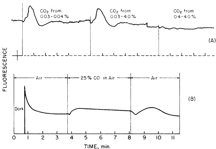
Fig. 33.37. Effect of changes of CO 2 concentration on fluorescence. (A) Wheat; high light intensity (after McAlister and Myers 1940). (B) Hydrangea (after Franck, French and Puck 1941).
