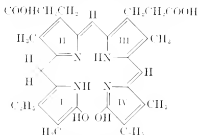
(I) Seidel's mesobiliviolin (= phycocyanobilin?)
