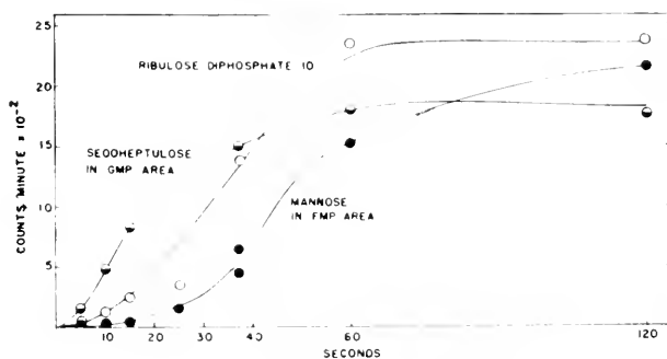
Fig. 36.17. C^{14}O_2 fixation in sedoheptulose phosphate, ribulose diphosphate, and mannose phosphate as function of time. 10 \mu l. Scenedesmus cells, 20° C. The separation of sedoheptulose and mannose is imperfect (both occurring in the same general monophosphate area) (after Benson et al. 1952).
