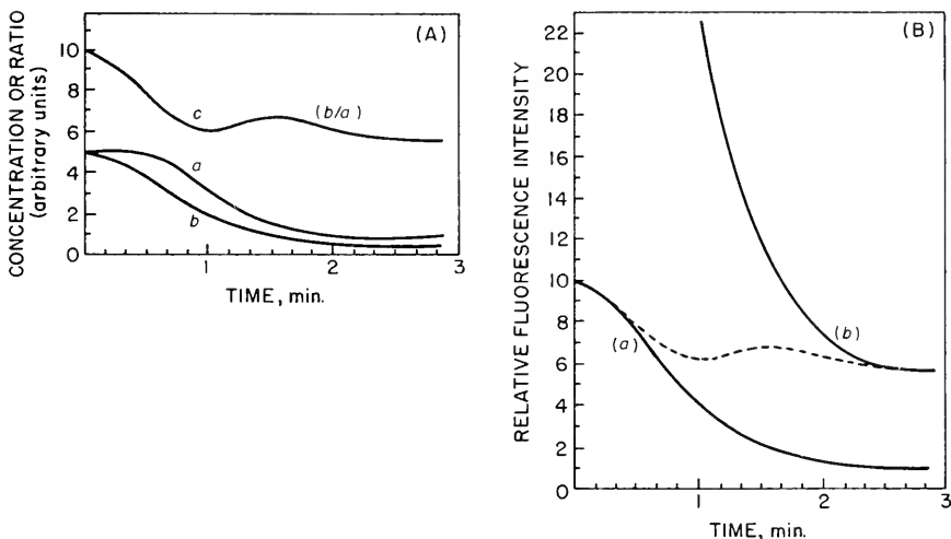
Fig. 33.50. Explanation of the second wave by competition of reducible substances and inhibitor for chlorophyll (after Shiao and Franek 1947): (A) concentration variation of narcotics ( b ), of photosynthetically reducible substances ( a ) and of their ratio; (B) theoretical fluorescence-time curves at two concentrations of photosensitive reducible substance, with transition curve shown as broken line.
