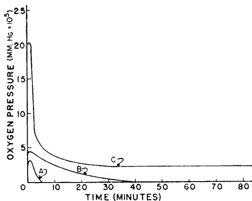
Fig. 35.19A. Photochemical O_2 evolution from 3 mm. 3 of separated spinach chloroplasts (A) and from crude leaf juice (B,C), both containing 3 \mu g. Chl (Tolmach 1951). Phosphoroscopic determination of O_2 pressure in N_2 gas flow (9.6 cm. 3 N_2 /min.), 10–12° C.
