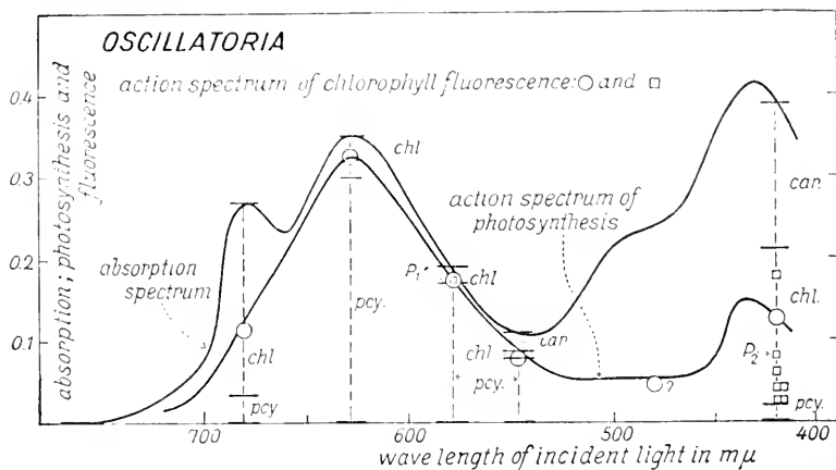
Fig. 37C.51. Absorption and action spectra of Oscillatoria (after Duysens 1952). At 680, 630, 578, 546 and 420 m\mu , the contributions of chlorophyll a (chl.), phycocyanin (pcy.), and carotenoids (car.) to total absorption (upper curve) are indicated. Lower curve: action spectrum of photosynthesis; points (O) indicate action spectrum of chlorophyll fluorescence in an algal layer with negligible absorption. Points at \lambda 578 and 420 m\mu , designated \square , were determined in a different way, and with various cultures. (At 578 m\mu both points were made to coincide with the action spectrum of photosynthesis.)
