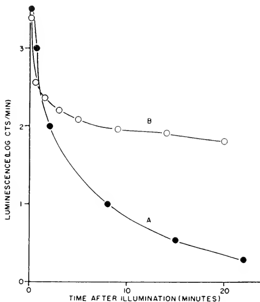
Fig. 37C.23A. Decay of "photosynthetic luminescence" at 25^{\circ}\text{C} . (after Strehler 1951). Curve A: Spinach, mustard leaf, Chlorella , spinach chloroplasts, washed mustard chloroplasts. Curve B: Unwashed mustard chloroplasts.
