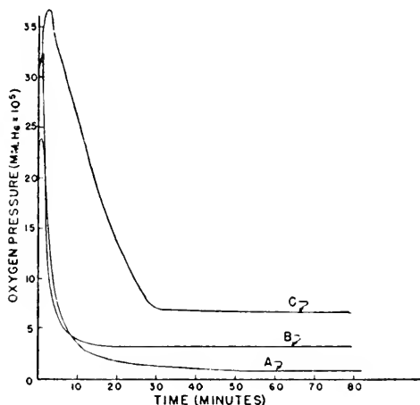
Fig. 35.19C. Photochemical O_2 evolution from 1.5 mm. 3 chloroplast suspension (1.5 \mu g. Chl) to which were added: (A) 1.5 mm. 3 water; (B) 1.5 mm. 3 1 \times 10^{-3} M TPN; (C) 1.5 mm. 3 1 \times 10^{-2} M TPN. 10-12^\circ C.; 9.4 cm. 3 N_2 /min. (Tolmach 1951).
