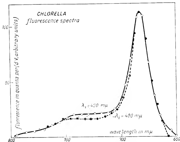
Fig. 37C.49. Fluorescence spectrum of Chlorella excited at \lambda_1 420 and 480\text{ m}\mu (the latter appreciably absorbed by chlorophyll b ) (after Duysens 1952). The fluorescence peaks are at 683\text{ m}\mu , slightly beyond the main absorption peak of Chlorella at 680\text{ m}\mu . No fluorescence peak is noticeable slightly beyond the absorption peak of chlorophyll b at 650\text{ m}\mu . (Corrected for re-absorption of fluorescence in the cells.)
