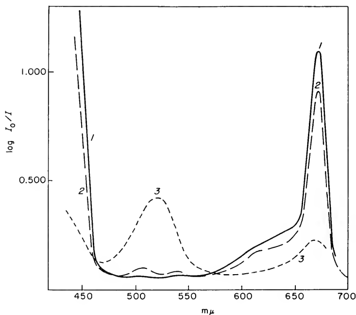
Fig. 35.3. Reversible reaction of chlorophyll a with ascorbic acid in pyridine in light (after Krasnovsky 1948): (1) spectrum before reaction; (2) spectrum after reaction; (3) approximate spectrum of the unstable reaction product (6 min. after darkening).
