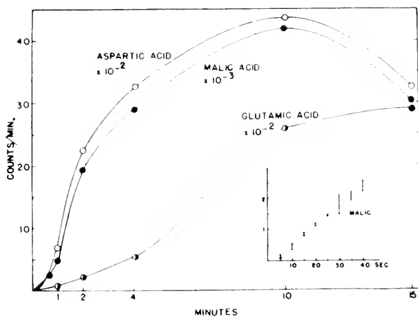
Fig. 36.18. C^{14}O_2 incorporation in some C_4 compounds as function of time (10 \mu l. Scenedesmus , 15° C.). Insert shows the initial slope of the malic acid tagging curve (after Benson et al. 1952).
