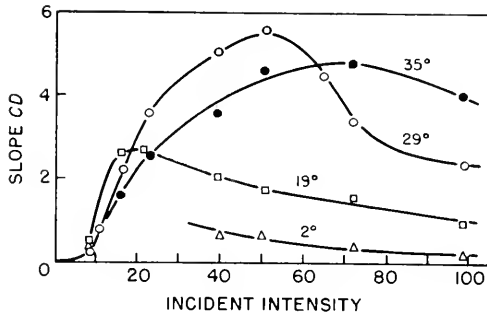
Fig. 33.41. Slope of second fluorescence wave as function of light intensity at various temperatures (after Wassink and Katz 1939). Gas phase, air; total inhibition of photosynthesis by cyanide.
