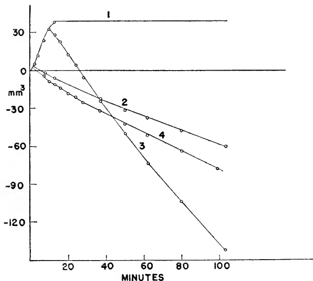
Fig. 35.17A. Evolution and absorption of O_2 by chloroplast material (300 \mu\text{g} . chlorophyll in 2 ml. phosphate buffer pH 6.8) (Mehler 1951). O_2 evolved in vessel 1 ( 5 \times 10^{-6} mole quinone); O_2 consumed in vessel 2 (4 mg. catalase, 10^{-3} mole ethanol); O_2 first evolved, then consumed at double speed in vessel 3 (5 \mu\text{mole} quinone, 4 mg. catalase, 10^{-3} mole ethanol). Vessel 4; catalase, ethanol, and 5 \mu\text{mole} hydroquinone.
