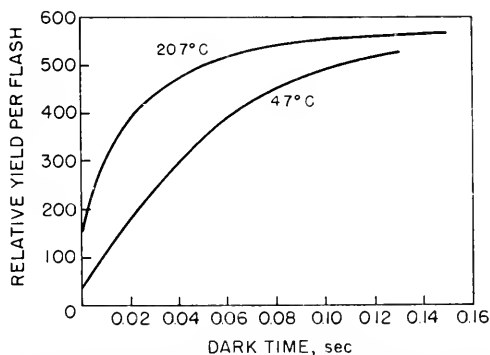
Fig. 34.14. Yield per flash curves for low and high temperature (after Weller and Franck 1941).
