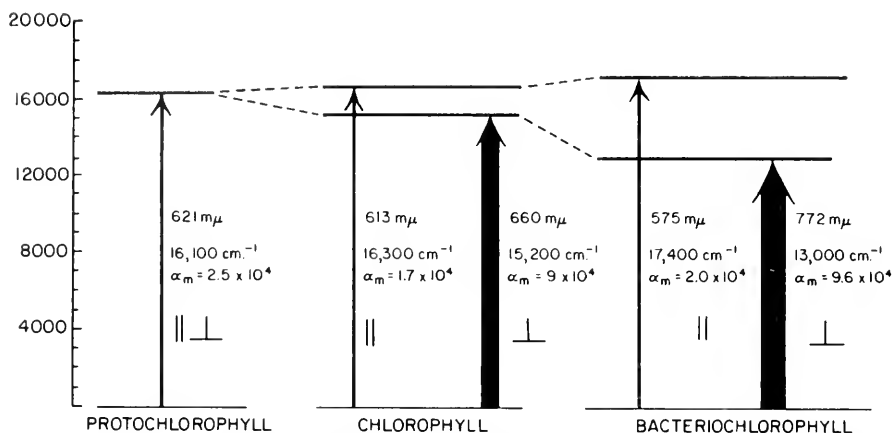
Fig. 37C.2. Low frequency bands of protochlorophyll, chlorophyll a , and bacteriochlorophyll (in ether). The symbols || and ⊥ refer to the long axis in bacteriochlorophyll and the corresponding direction in chlorophyll (which is not a symmetry axis).
