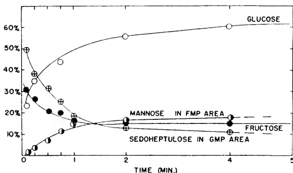
Fig. 36.21. Distribution of C(14) label between several sugars as function of time of photosynthesis ( Scenedesmus , 15° C.) (after Benson et al. 1952).
