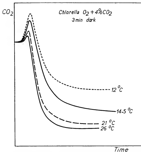
Fig. 33.13K. \text{CO}_2 burst in Chlorella at different temperatures; diaferometer record (after van der Veen 1950).
