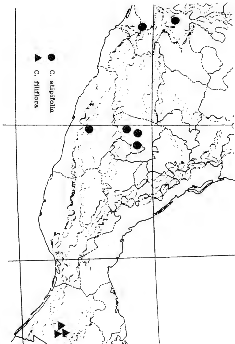
Map 5. Distribution of Castilleja stipifolia and C. filiflora .
