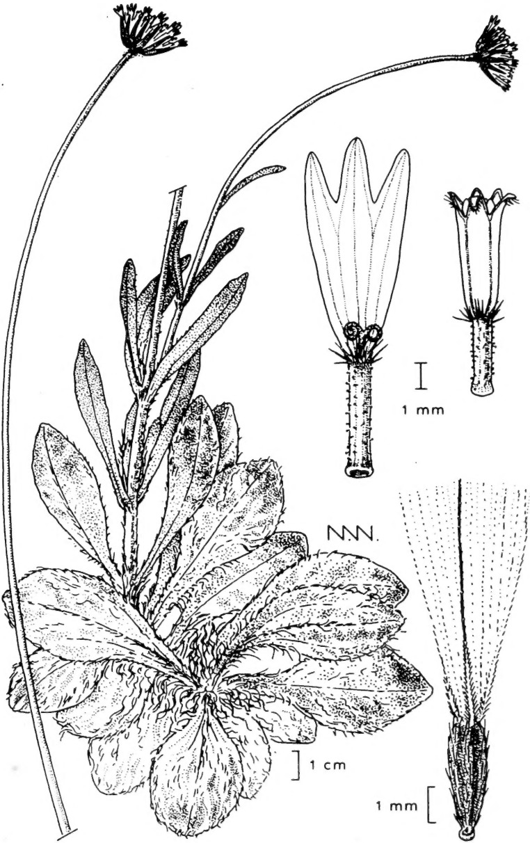
Fig. 1. Tridax hintoniolum , from holotype.
