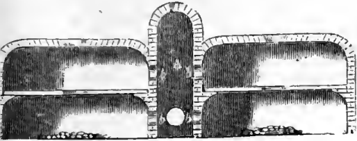
1722.—Egyptian Egg-Oven.
