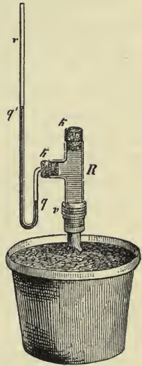
FIG. 172. — Apparatus for measuring root pressure. To the stump of a plant a T-tube, R , is attached by a piece of rubber tubing, v . The other openings are closed by rubber corks, k , through one of which passes a small glass tube, r , bent into two unequal legs, containing mercury. Through the upper should pass a short piece of glass tubing drawn out to a fine point, to be sealed off in a flame after R is filled with water. At the beginning of the experiment the mercury is about at the same level in both legs. As water is forced from the stump into R by root pressure the mercury rises in the arm r' and falls correspondingly in r .—After Sachs.
