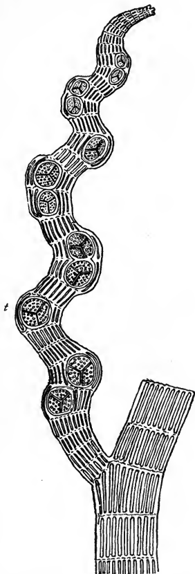
FIG. 229.—A branch of a red seaweed ( Polysiphonia opaca ), showing tetraspores, t , formed by an internal cell of the thallus. Magnified about 100 diam.—After Kütz ing.
