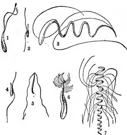
FIG. 306.—Sperms of various plants, showing variety of form. 1, Volvox aureus ; 2, Vaucheria synandra ; 3, Clava fragilis ; 4, Fucus serratus ; 5, Marchantia polymorpha ; 6, Equisetum Telmateia ; 7, Marsilia vestita . Magnified 1000 diam.—After Möbius.
