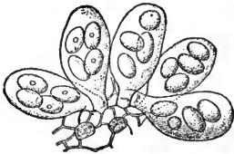
FIG. 224.—A cluster of asci from the interior of the fructification of a mildew ( Erysiphe Heraclei ) similar to those shown in fig. 223. Each ascus contains four spores. Magnified 200 diam.—After DeBary.
