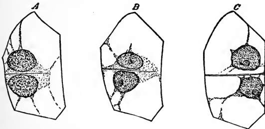
FIG 22B.—Three stages of division in the same cell of an orchid ( Epipactis palustris ). The cell is occupied in great part by vacuoles. In this case the new wall forms first on one side between the nuclei ( A ), which gradually travel across to the opposite side ( B ), the wall extending until it is complete ( C ). Magnified about 380 diam.—After Treub.
