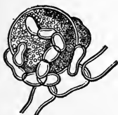
FIG. 377.—Hyphæ of a lichen, Cladonia furcata (see fig. 55), enveloping an alga, Protococcus . Magnified 950 diam.—After Kerner.
