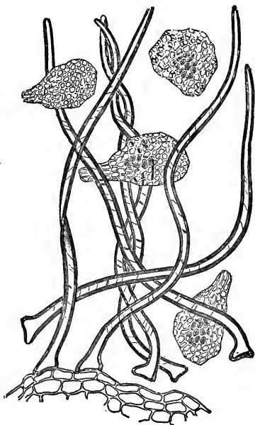
FIG. 407.—Seeds of an orchid ( Vanda teres ), with cells of seed coat bladdery and filled with air. These seeds are ejected from the capsule by the contortions of the hairs on its inner faces which curve and twist as the moisture in the air varies. Magnified 100 diam.—After Kerner.
