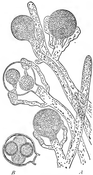
FIG. 336.—A. Functionless sex-organs of a fungus ( Achlya lignicola ). Ovaries globular, with 2-4 eggs; spermarium from branches of same hypha form fertilizing tube which remains closed. B, eggs which have become resting spores without fertilization. Magnified 265 diam.—After Sachs.
