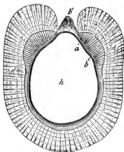
FIG. 209.—Section of a mature spore of Pilularia globulifera . h , the cavity of the cell (contents not shown); a , the true wall; b the first, c the second, d the third layer of the epispore. b forms a papilla at b' . c and d have a prismatic structure. Magnified about 50 diam.—After Sachs.
