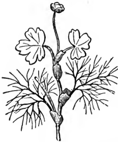
FIG. 187.—A shoot of water crowfoot ( Ranunculus aquatilis ). The lower leaves have developed under water and are branched into many narrow divisions; the two upper leaves have developed in air and at maturity float on the surface of the water. About half natural size.—After Frank.
