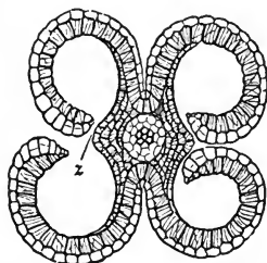
FIG. 263.—Transverse section of bursted anther of a lily ( Betonium umbellatus ). Sporangia have ruptured at z , so that the two pairs have each formed a single cavity. The connective is relatively small; in the center a single stele. Magnified about 20 diam.—After Sachs.
