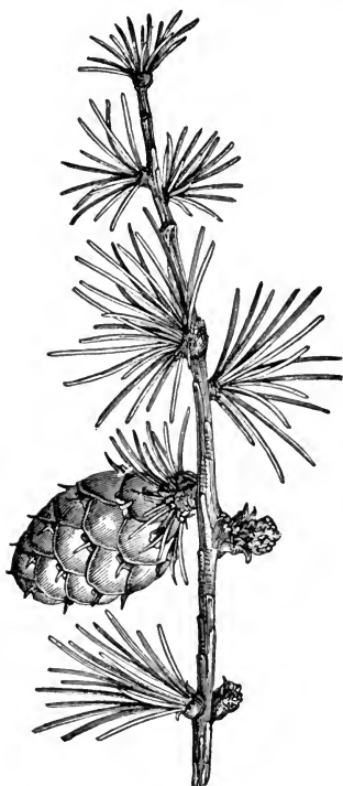
FIG. 358.—Shoot of larch, with ripe cone; showing needle-shaped leaves on dwarf branches; scale leaves on main axis; carpellary scales just peeping from between placental scales of cone. Natural size.—After Kerner.
