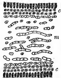
FIG. 45.—Diagram of a portion of fig. 44, magnified about 70 diam. c , cortex; m , medulla. The varied forms of the cells are due to the different planes in which the filaments are cut. The clear spaces are filled with mucilage produced by the cell-walls. From a drawing by Mr. C. E. Allen.
