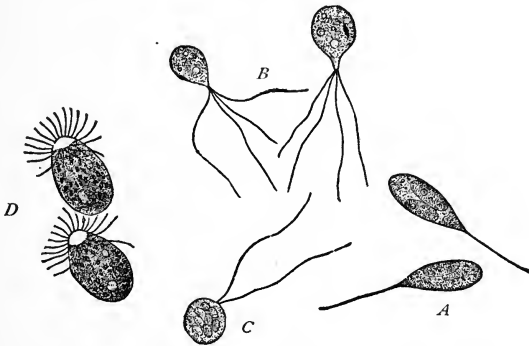
FIG. 168.—Zoospores of various forms, swimming in water by means of one or more cilia. A, Botrydium ; B, Draparnaldia ; C, Coleochaete ; D, Edogonium . Highly magnified.—After Kerner.
