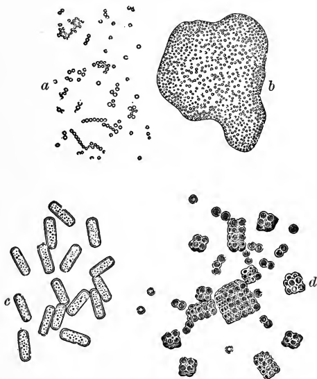
FIG. 16.—Various bacteria. a , Micrococcus , the "blood-portent"; b , zoogloea form of the same; c , Bacterium aceti , the ferment of vinegar; d , Sarcina , a harmless parasite of the human intestine. a , b , magnified 300 diam.; c , 2000 diam.; d , 800 diam.—After Kerner.
