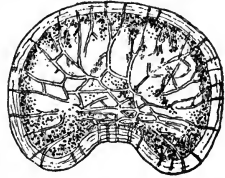
FIG. 33. - Transverse section of axis of Caulerpa , showing cross-bars to stiffen wall. Magnified about 25 diam.— After Murray.
