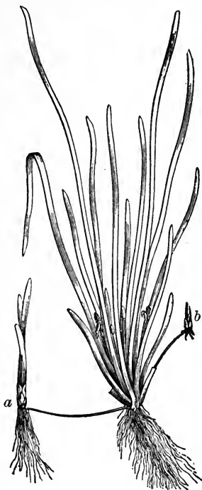
FIG. 298.—A plant of eel-grass ( Vallisneria spiralis ) forming new plants, a , b , at tips of runners, arising from axils of lower leaves. One third natural size.—After Schinzlein.
