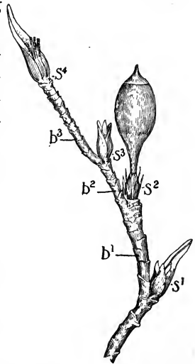
FIG. 71.—Axis of a moss ( Orthotrichum ) showing sympodial branching. S^1, S^2, S^3, S^4 , successive clusters of sexual organs, produced at apex which check the growth of axis. Beneath each a lateral growing point develops, producing successively the branches b^1, b^2, b^3 . Magnified 10 diam.—After Bruch & Schimper.
