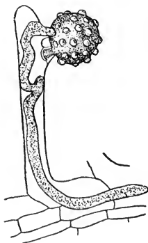
FIG. 248.—One of the hairs from the stigma of corn cockle ( Lychnis githago ) to which a pollen grain adheres. The pollen tube has penetrated the hair and is making its way down the style. Magnified 175 diam.—After Strasburger.
