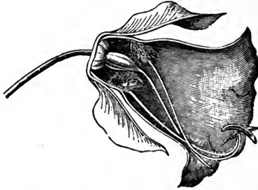
FIG. 403.—Flower of Cobæa scandens , halved; showing tufts of hairs on the base of the filaments, of which there are five; these close the bottom of the corolla cup where nectar is secreted against intruders. Three-fifths natural size.—After Kerner.
