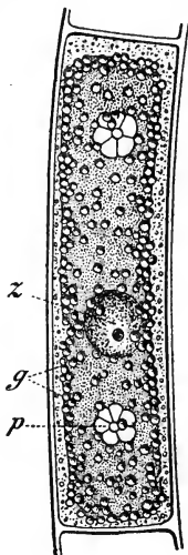
FIG. 27.—A cell from filament of Mesocarpus . The darker body nearly filling cell is the chloroplast (face view) in which are pyrenoids, p , and tannin vesicles, g . If seen from a direction at right angles it would appear as a narrow stripe in the center of the cell. z , the nucleus. Magnified about 200 diam.—After Zimmermann.
