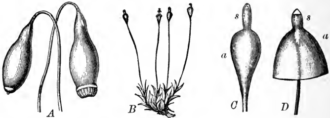
FIG. 72.—A, two capsules of Bryum ; from the right-hand one the lid has fallen, showing the teeth. Magnified 5 diam. B, four gametophyte shoots of Splachnum ampullaceum , bearing four sporophytes. Natural size. C, a capsule of one of the same sporophytes, showing enlarged apophysis, a , below the sporangium, s . Magnified 10 diam. D, capsule of Splachnum luteum , with umbrella-like apophysis, a , below sporangium, s . Magnified 2 diam.
