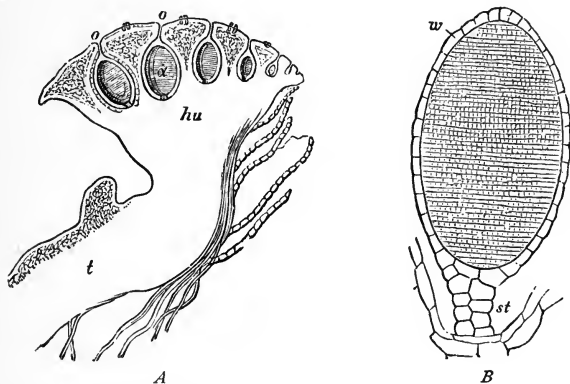
FIG. 311.— A , a longitudinal section of a male head of Marchantia . t , portion of thallus; hu , enlarged head or receptacle; a , spermaries, sunk in pits opening at o . Magnified about 15 diam. B , compound spermary. w , its wall, surrounding the immense number of minute regularly arranged sperm mother cells; st , its stalk. Magnified about 80 diam.—After Sachs.
