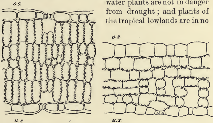
FIG. 31. Sections through leaves of the same plant, showing the effect of exposure to light upon the structure of the mesophyll. In both cases o.s. indicates upper surface, and u.s. under surface. In the section at the left the growing leaf was exposed to direct and intense sunlight, and, as a consequence, all of the mesophyll cells have assumed the protected or palisade position. In the section at the right the leaf was grown in the shade, and none of the mesophyll cells have organized in palisade fashion.—After STAHL.
