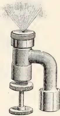
Graduating Vermorel Nozzle
