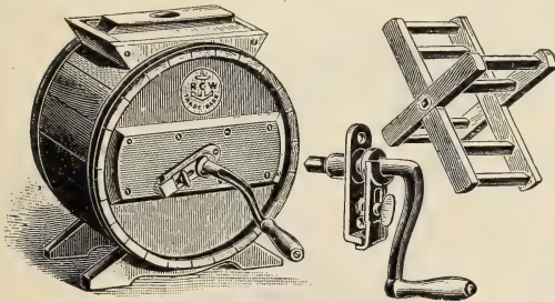
Double Dasher—Thumb Screw Lock.
