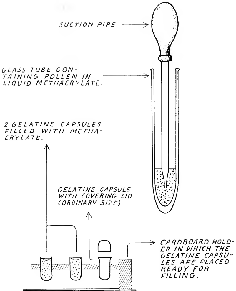
Fig. 254. Outfit for filling the gelatine capsules.
