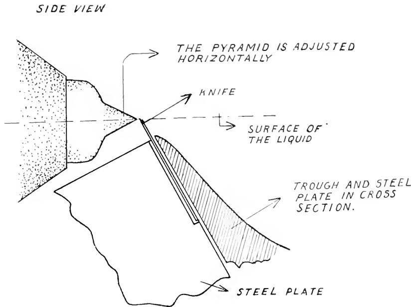
Fig. 264. Pyramid and part of trough, side view.
