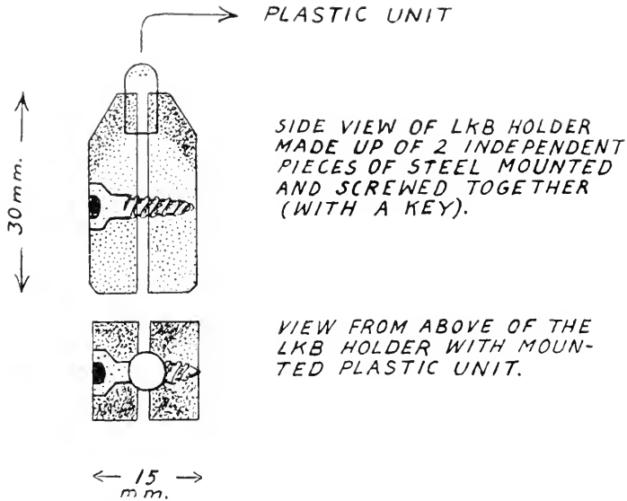
Fig. 256. LKB object-holder with plastic unit mounted (1:1).
