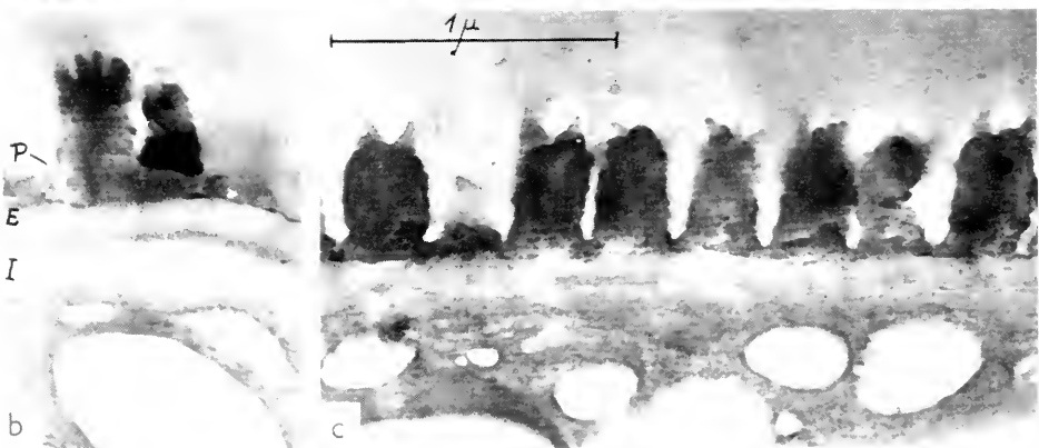
PL. IV. Fusaria hygrometrica . EMG D. von Wettstein. a, section through part of a spore; M, mitochondria; P, plastid. 23,000. b, oblique section of sporoderm (in line and two-layered exine) 34,000. c, radial (perpendicular) section through sporoderm; cytoplasm, intine, and exine closely connected. 34,000.
