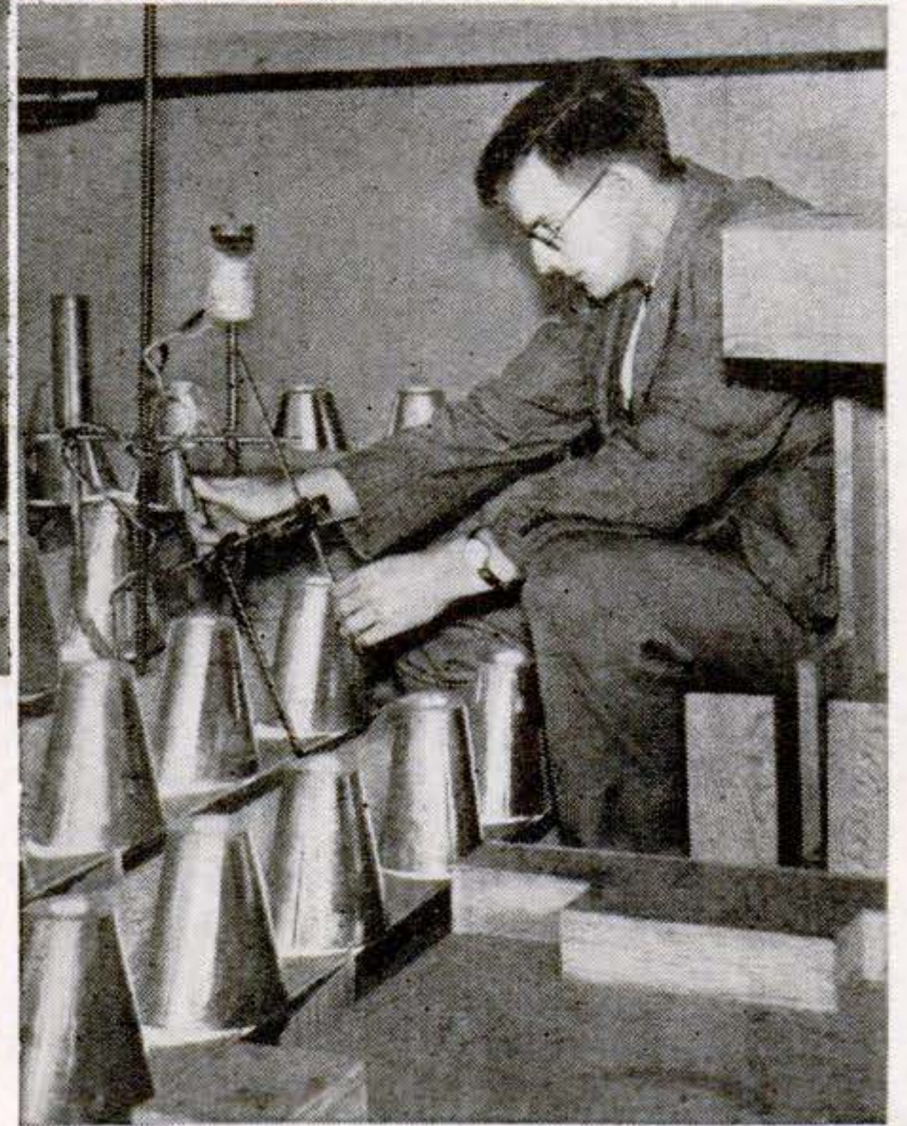
BETTER AIR FOR COMMONS. The British National Physics Laboratory has built a model of half of a proposed debating chamber (above) for the new House of Commons to test the ventilation system. Each conelike lamp on the benches emits the body heat of two persons. The air inlet can be seen at left under the gallery. Inset: A physicist checks the temperature of a lamp.
