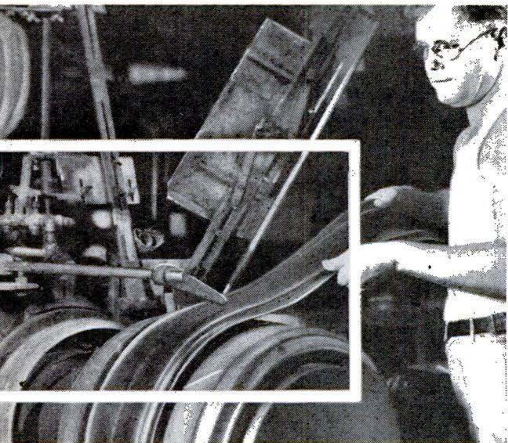
The old method of putting on a tread. Here again, besides being slower, the machinery allowed greater chances of human error and put most of the responsibility for quality on the operator.
