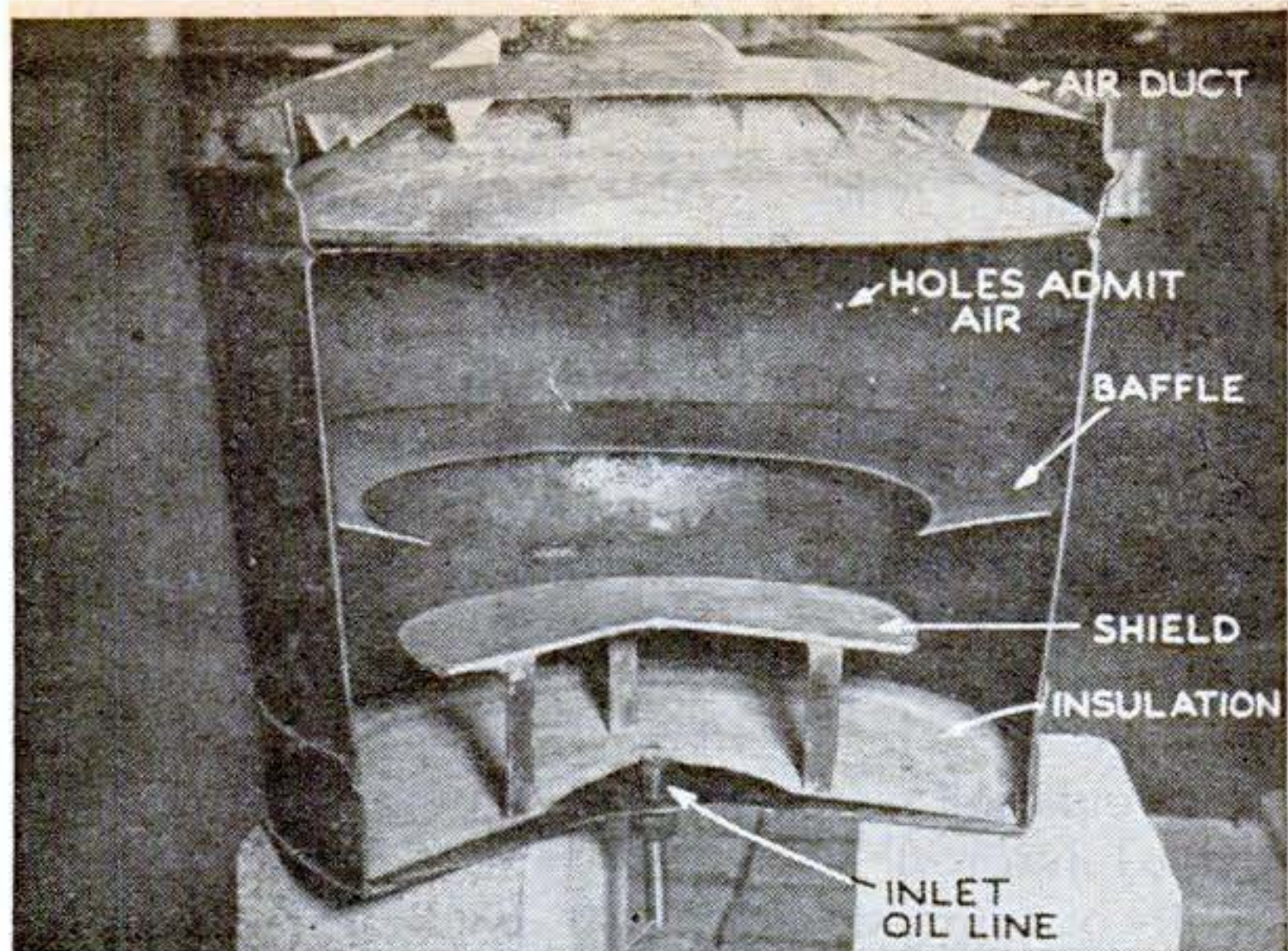
Ordinarily, pot burners require high grade oil because heat from the flame cracks a cheaper grade while it is vaporizing. Socony-Vacuum engineers now have developed a pot-type heater which prevents cracking, making it possible to use the more economical fuel. It is shown above under test and in a cutaway view.
