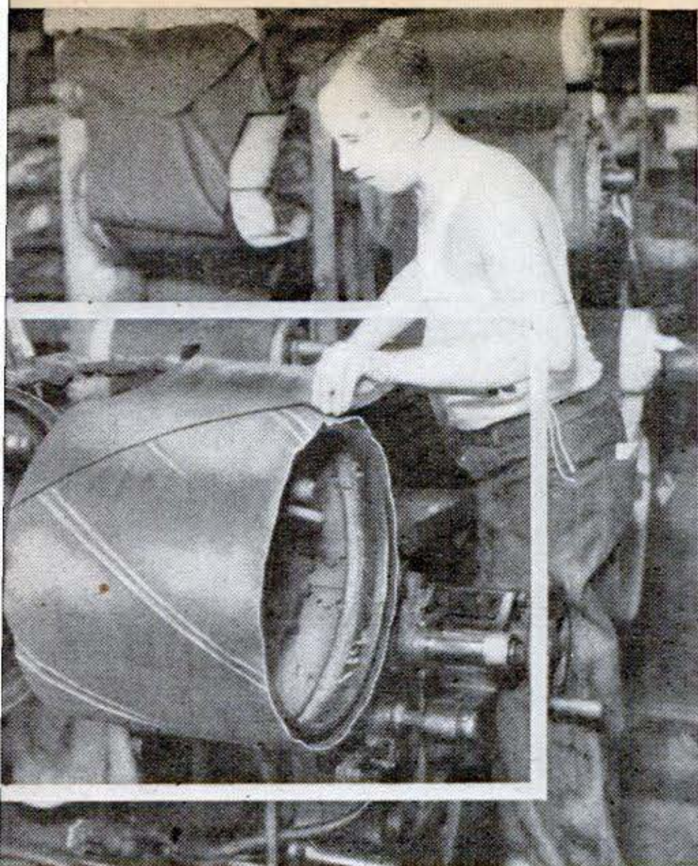
For contrast, here is the prewar system of laying on plies. With such machinery, finished product's quality depended largely on dexterity of operator.
