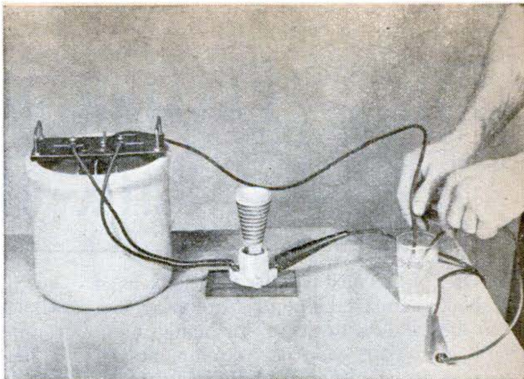
When both leads are submerged in a salt solution, bubbles will form around the negative wire. Short-circuit the wires to permit a hydroxide film to form on the aluminum plates.
