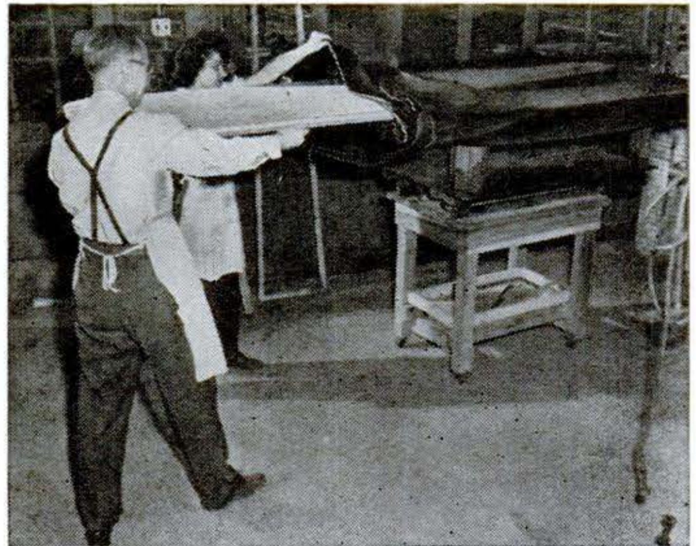
2. When enough of the resin-impregnated layers have been applied, the mold is put in a rubber bag for curing. Fiberglass materials, used in this process, meet all the varied demands of electronic heating.
