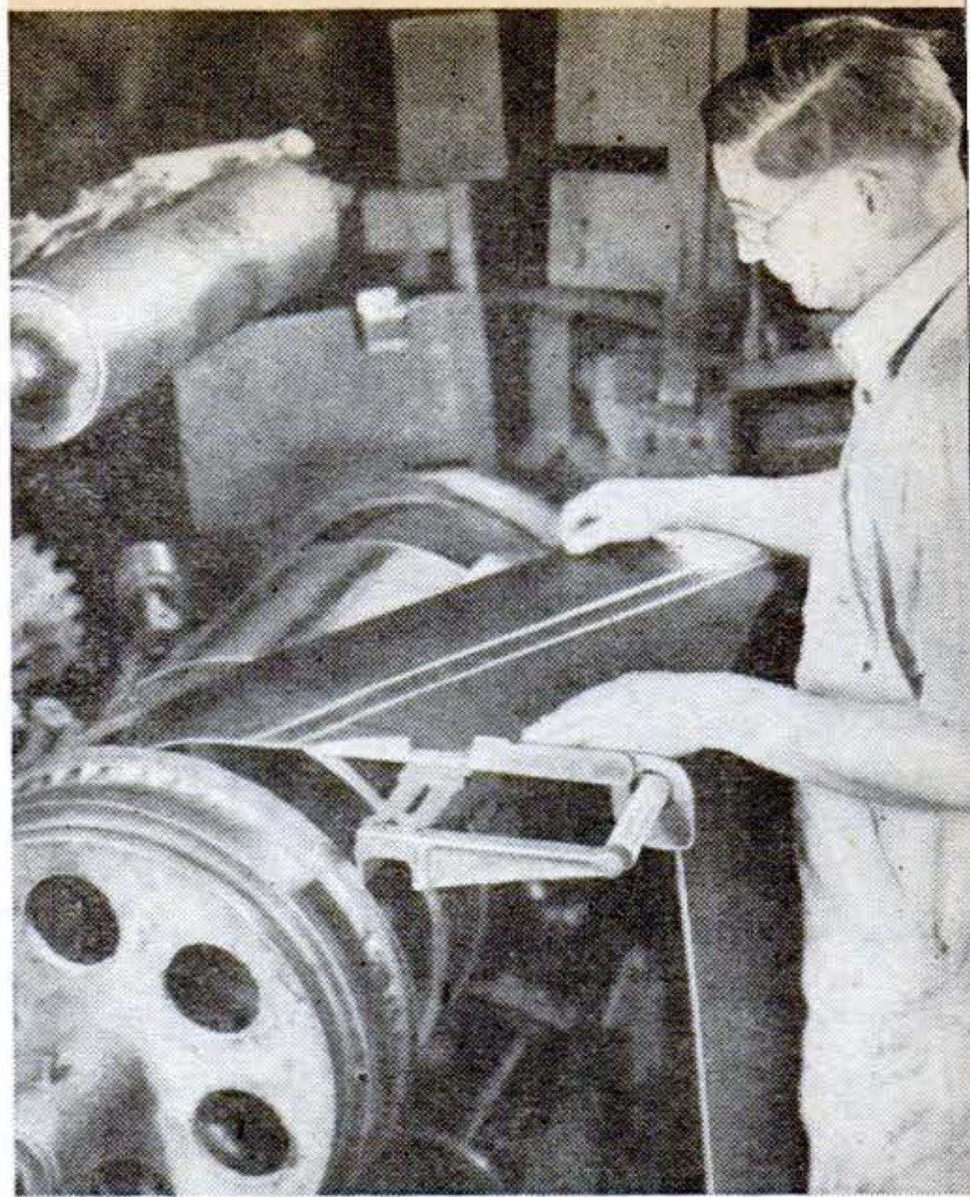
2. As the drum rotates, tire builder lays on first of fabric plies, cut on proper angle. This method assures uniform product, lessens emphasis on skill.
