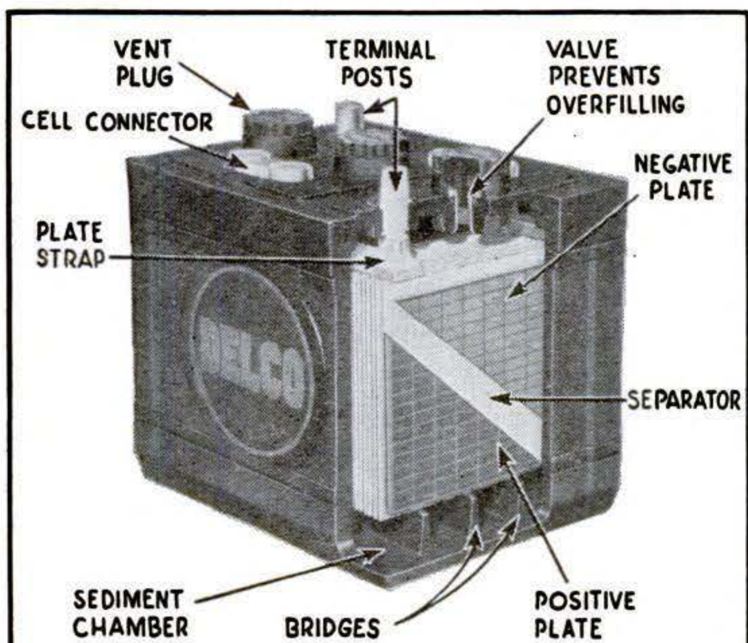
Here is a typical automobile storage battery, the end being cut away to show construction of one cell. How to use a hydrometer is shown below.
