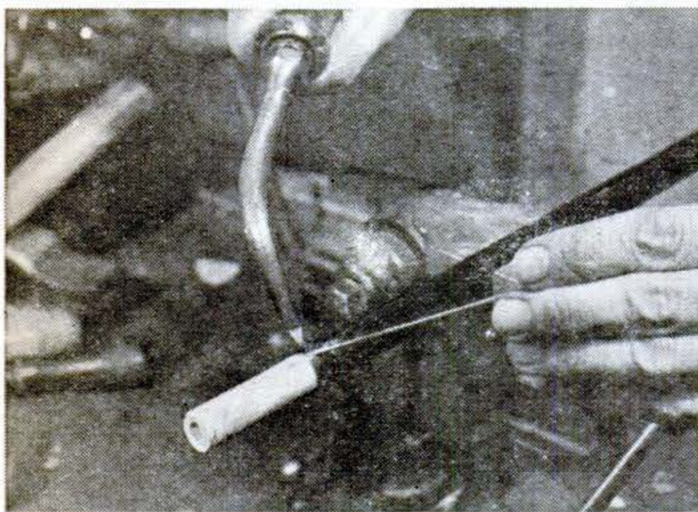
Splits in metal tripod legs are fixed by soldering the break over a porcelain tube and filing flush.
