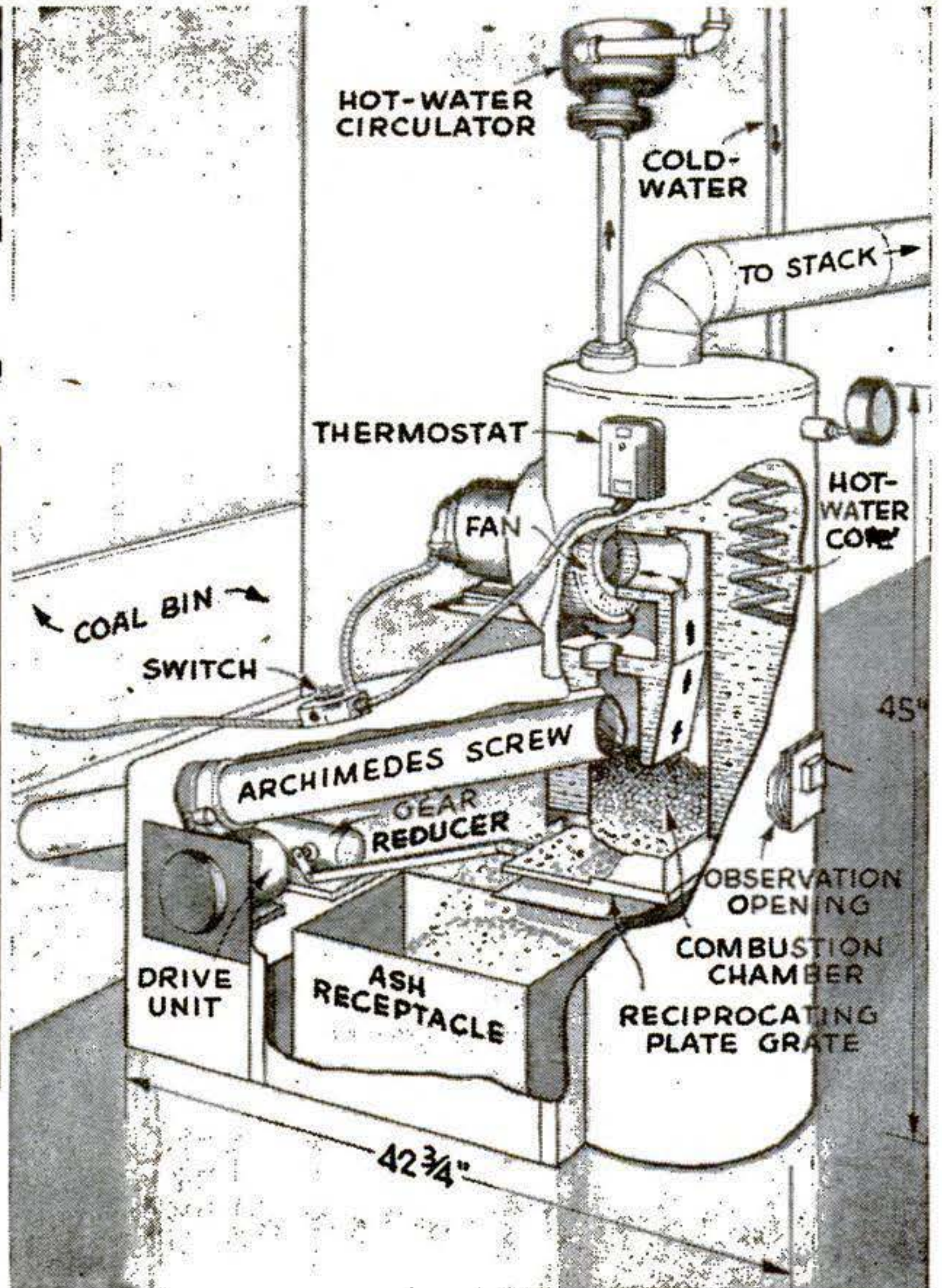
This midget furnace burns hard coal in a fire chamber only 8" in diameter. It was developed from the Anthratube, a pipelike, experimental heater announced two years ago. Fuel is fed by an Archimedes screw.
